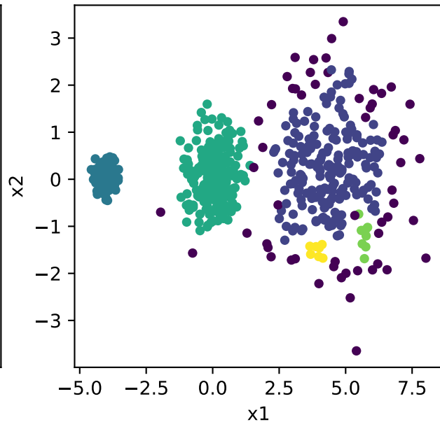
DBSCAN ARI = 0.84
