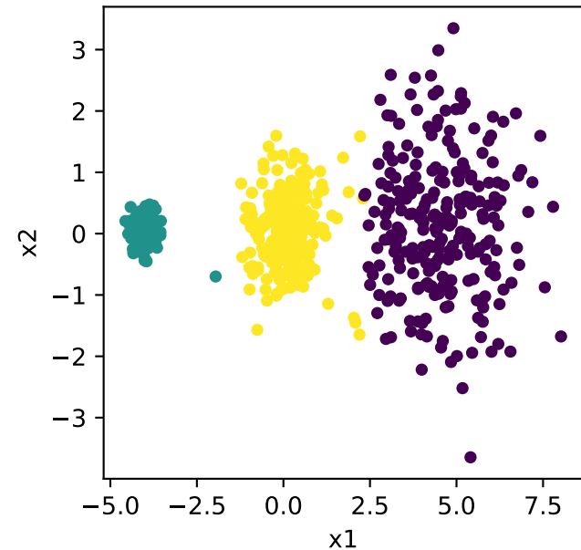
K-Means ARI = 0.96
