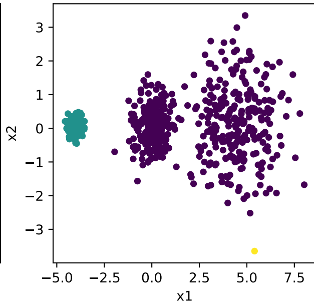
Unequal Densities Hierarchical: Single ARI = 0.51
