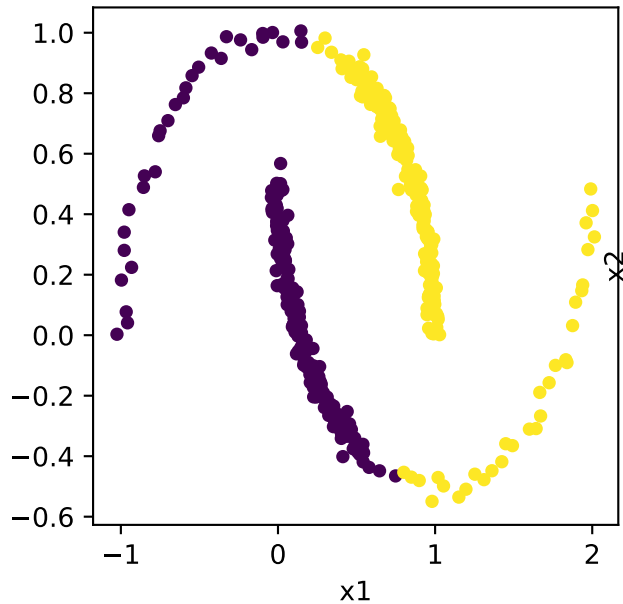
K-Means ARI = 0.49
