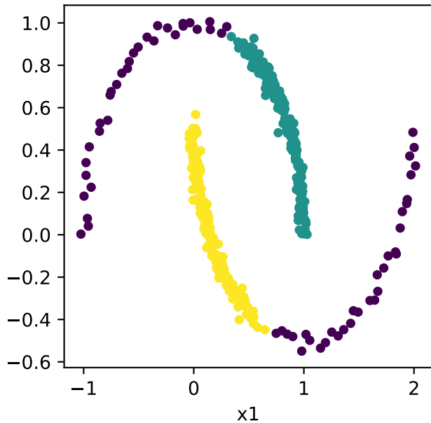
DBSCAN ARI = 0.71
