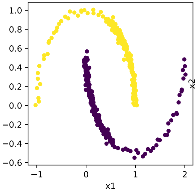
Uneven Chains Hierarchical: Single ARI = 1.00
