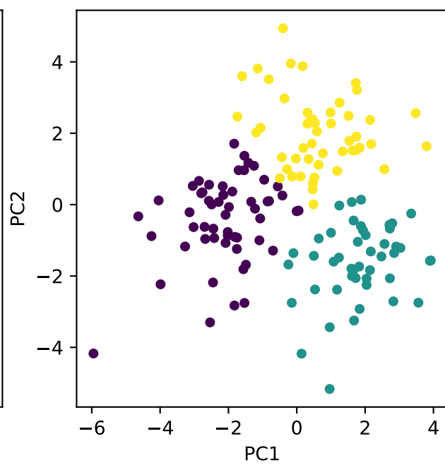
K-means After PCA
