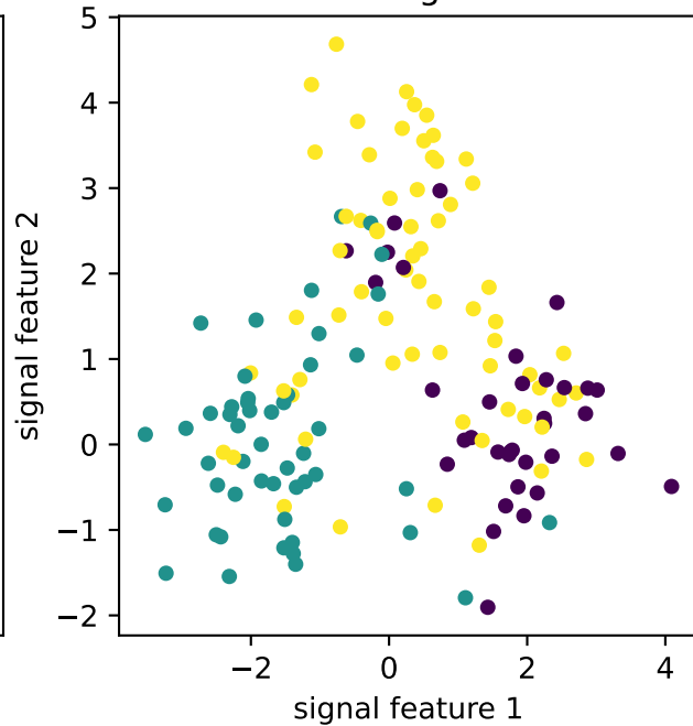
K-means on Original Features
