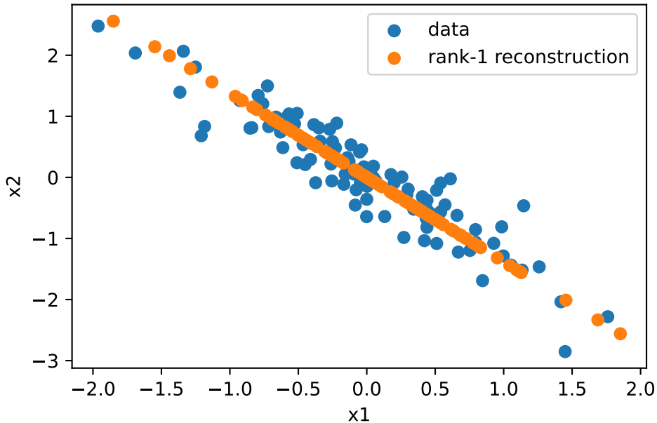
PCA Projection and Reconstruction
