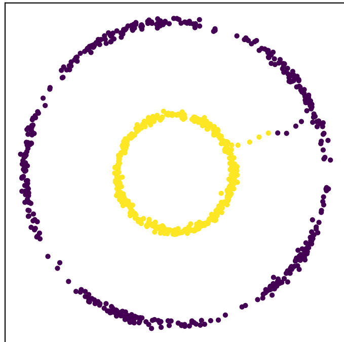
Spectral Clustering ARI = 1.000
