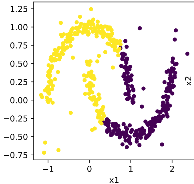
K-Means ARI = 0.20
