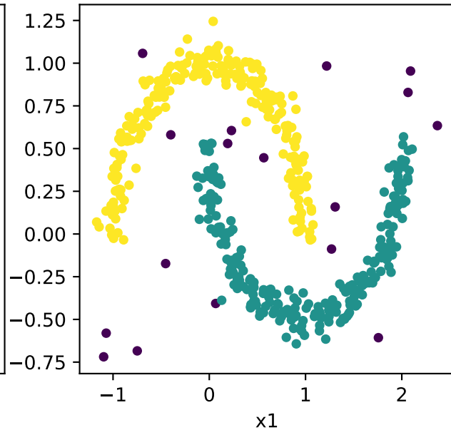
DBSCAN ARI = 0.94
