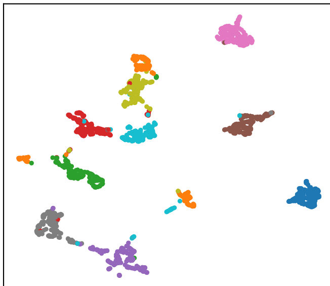
n_neighbors=15, min_dist=0.1
