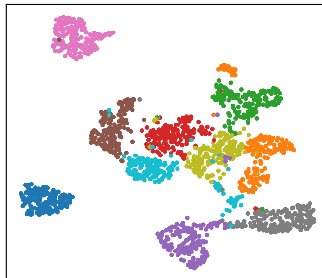
n_neighbors=50, min_dist=0.5
