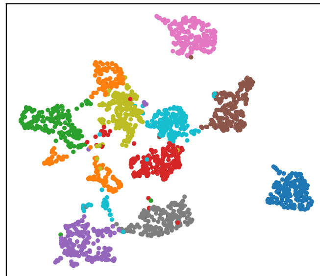
n_neighbors=15, min_dist=0.5
