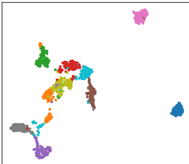
n_neighbors=50, min_dist=0.1
