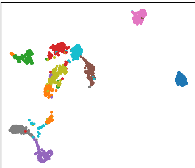
n_neighbors=50, min_dist=0.05
