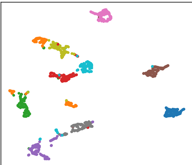
n_neighbors=15, min_dist=0.05
