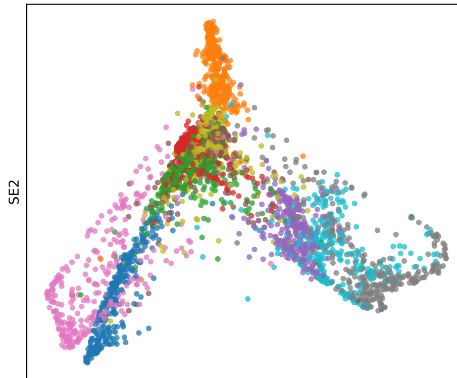
Spectral embedding
