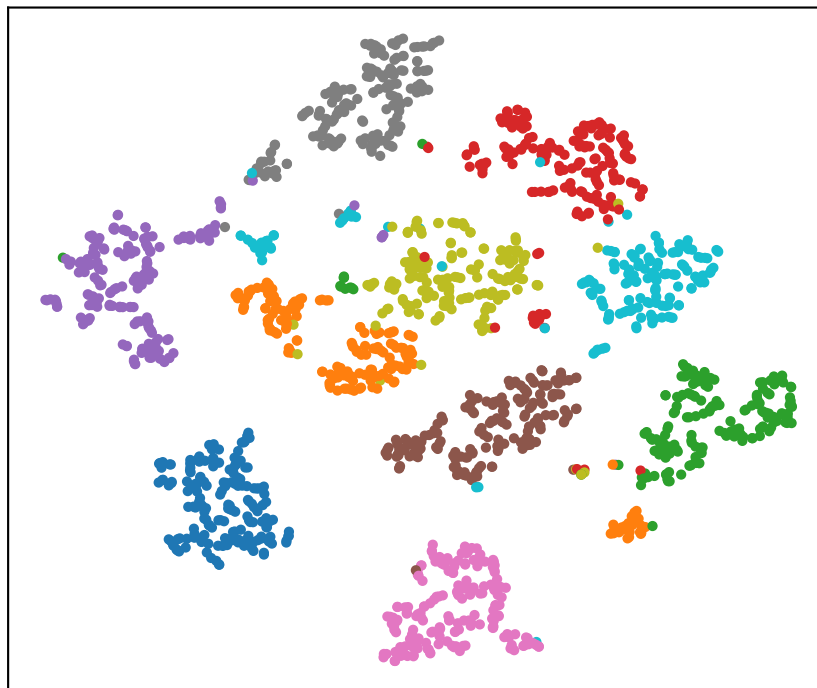
perplexity = 50
