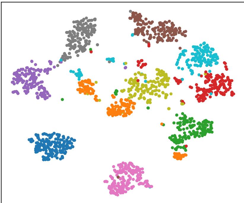
perplexity = 30
