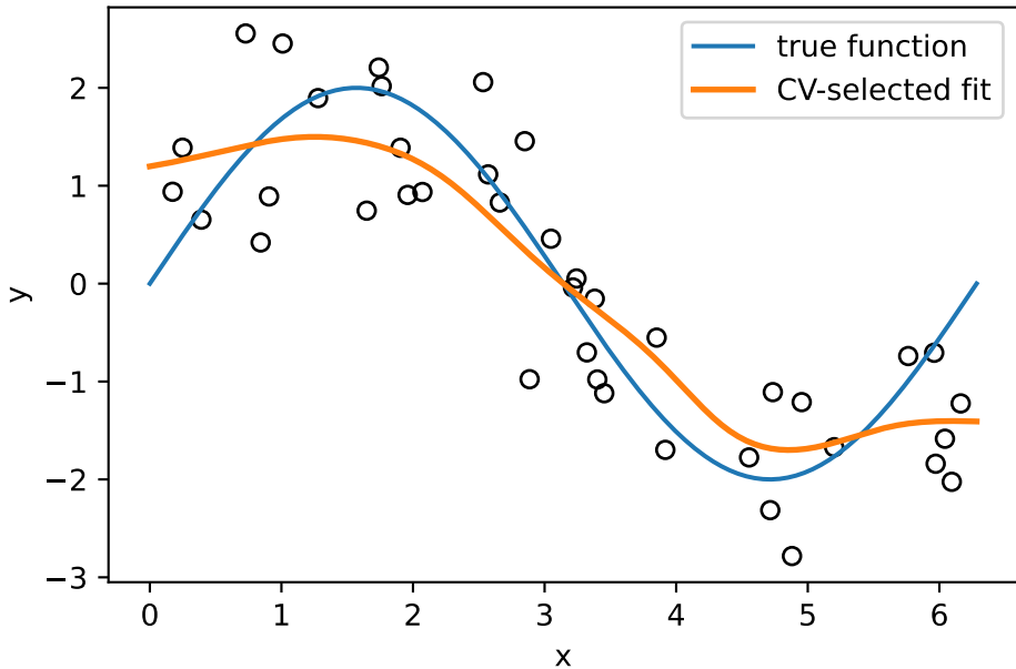
Selected Bandwidth = 0.53
