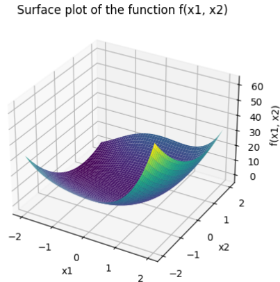
Figure 1: 3D plot of the function f(x_1, x_2)
