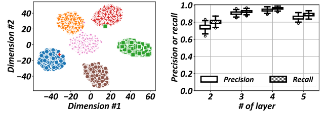
Figure 19: Impact of the number of sampling layer.
