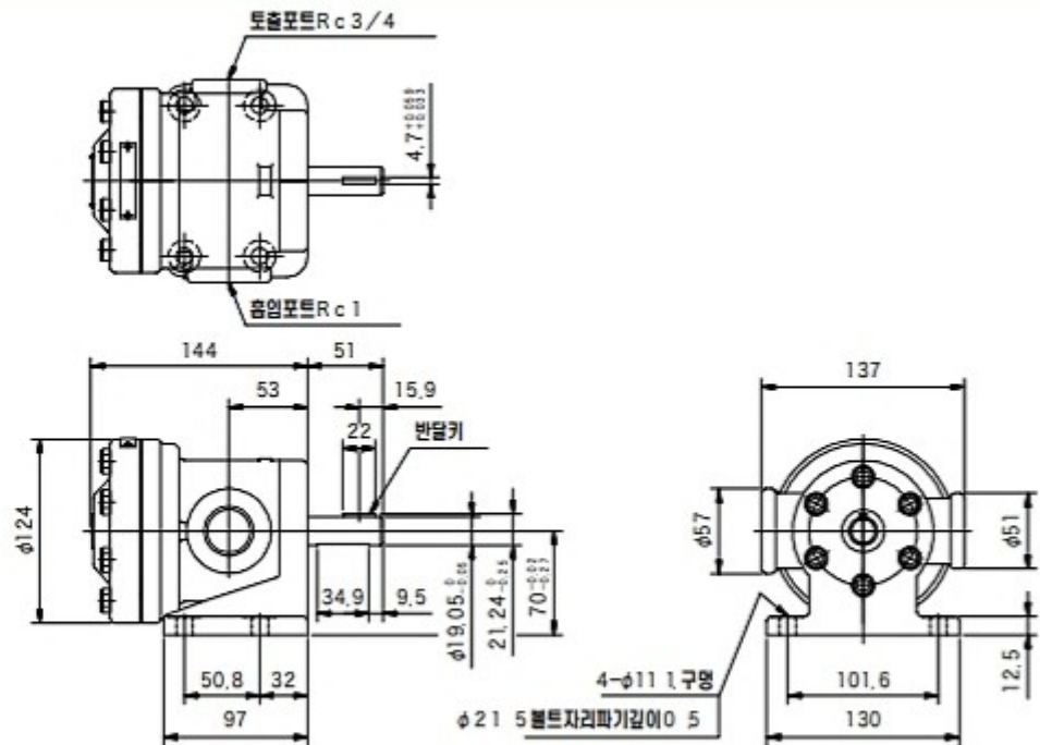
V-104 (FOOT 취부형)
