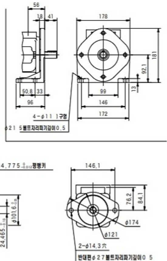
(FOOT 취부형)
