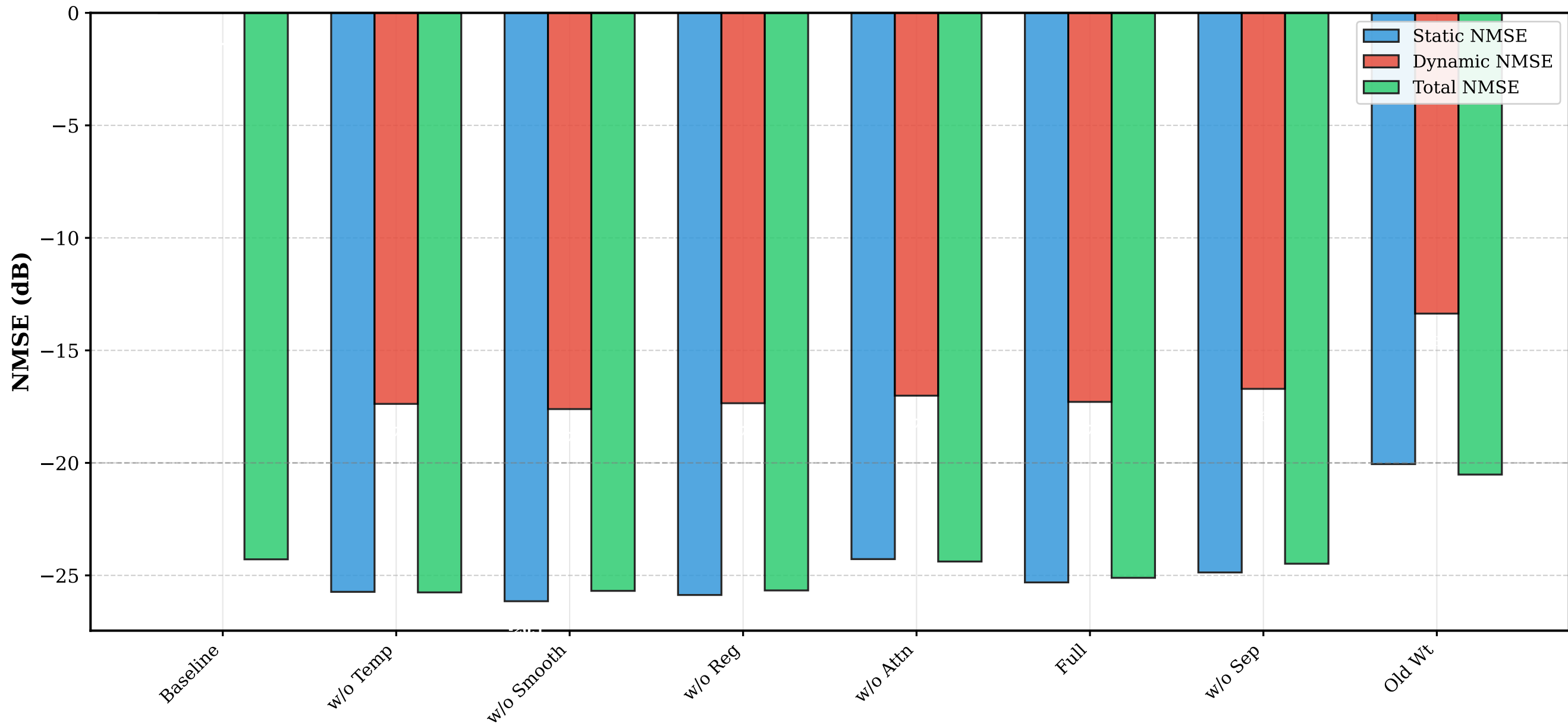
Normalized Mean Square Error Comparison
