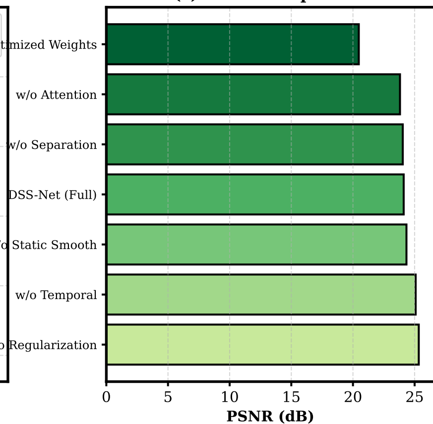
(c) PSNR Comparison
