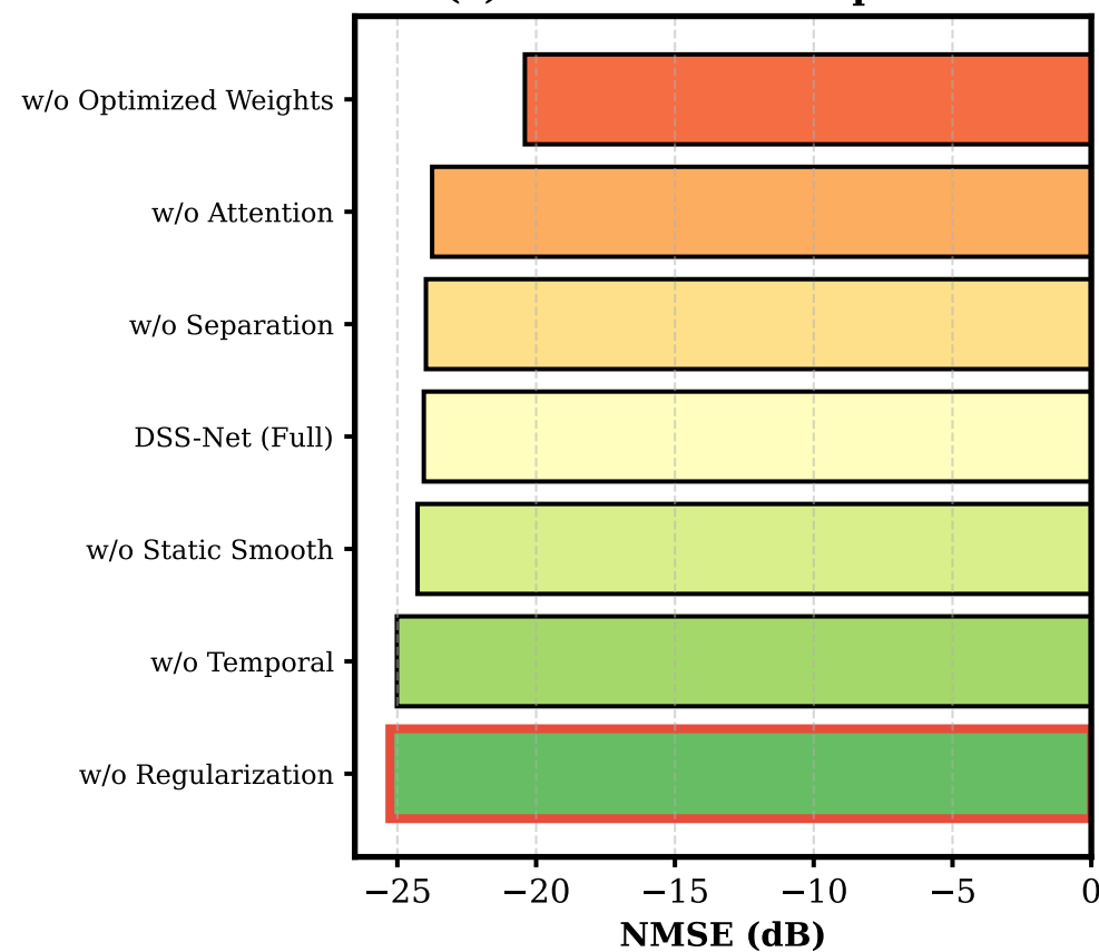
(a) Total NMSE Comparison
