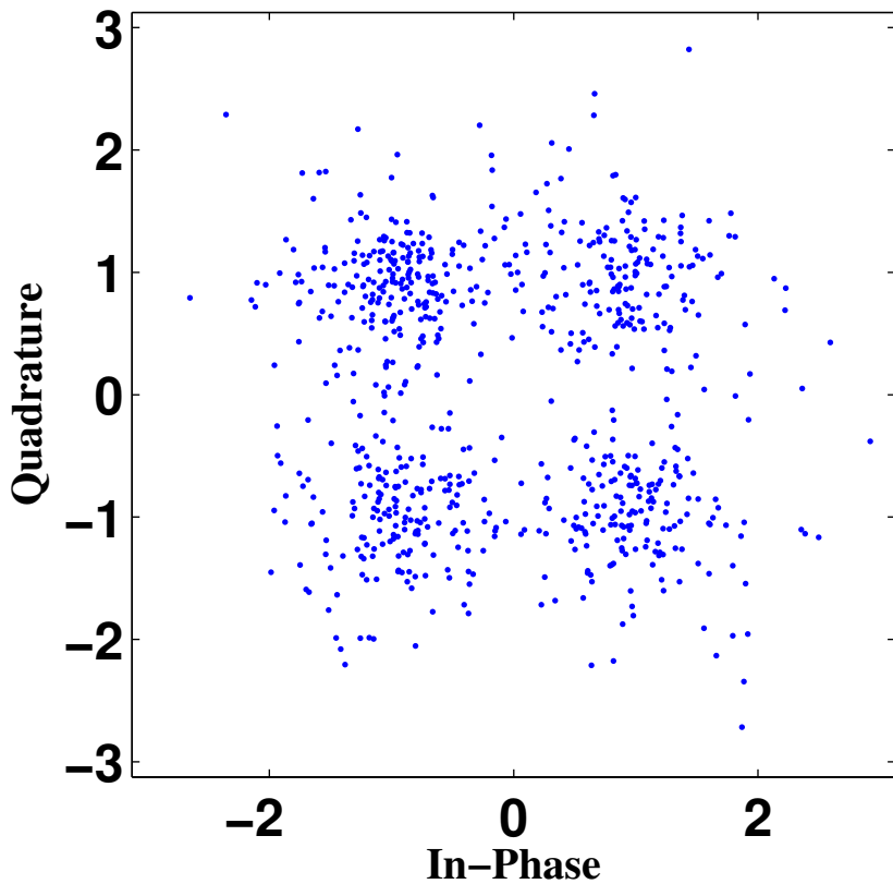
Scatter plot
