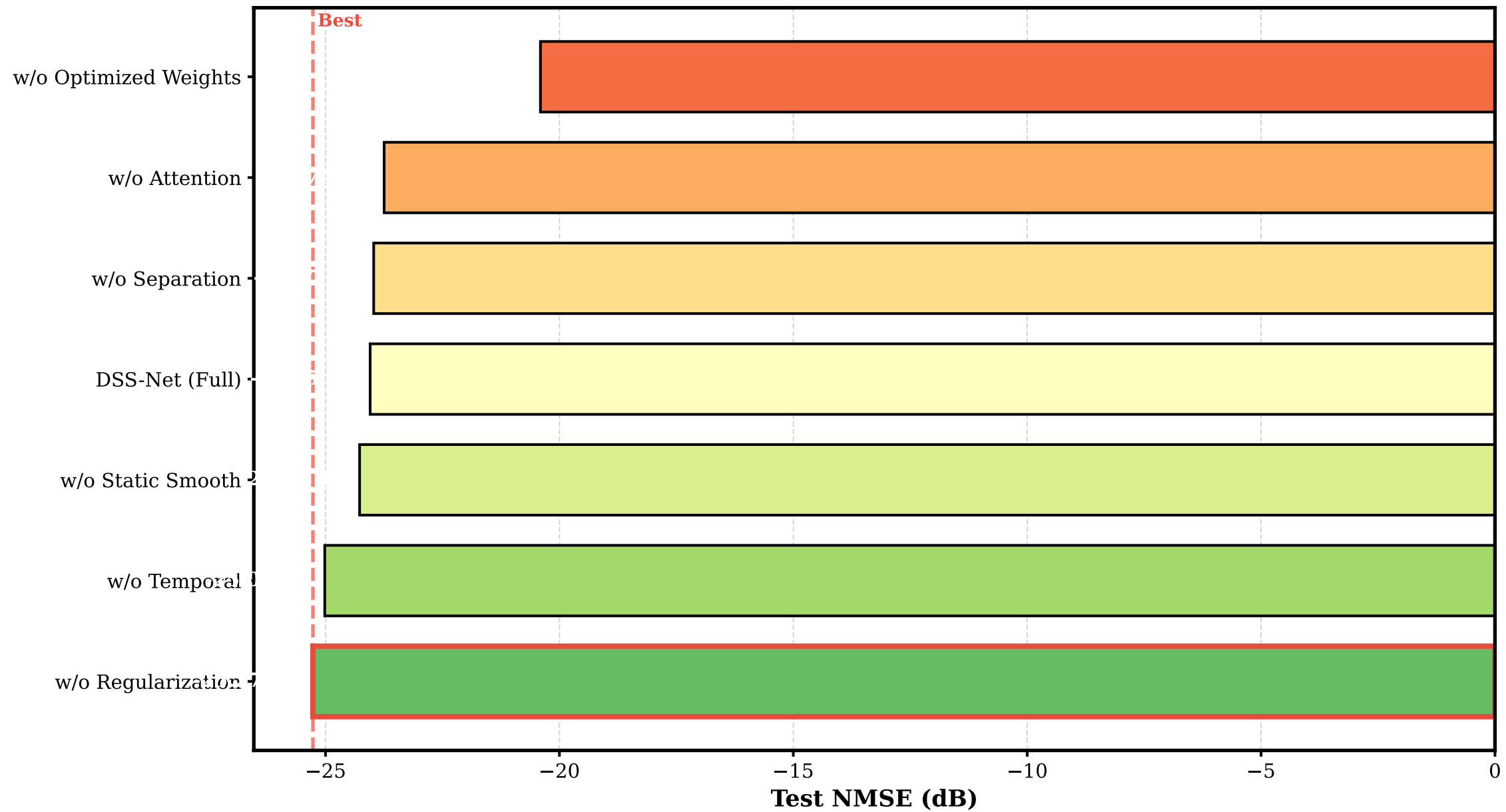
Ablation Study: NMSE Performance Comparison
