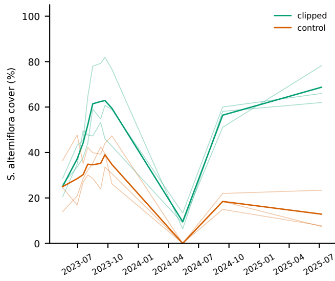
d Repeated clipping observations: 3 plots/arm
