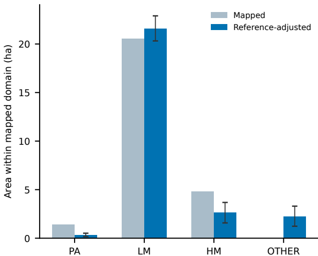
c Stratified reference-based area estimates
