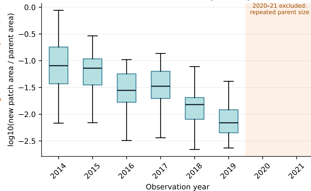
B Parent-normalized emergence signal
