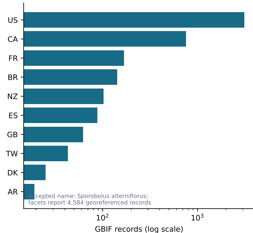
A Global occurrence context
