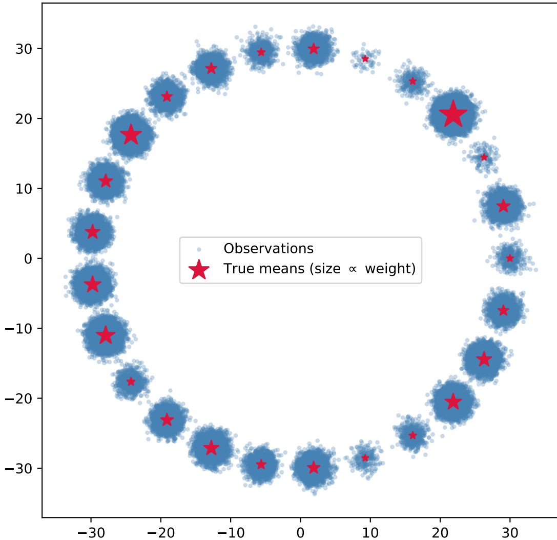
2D GMM data — n = 100000 samples, K = 25 components
