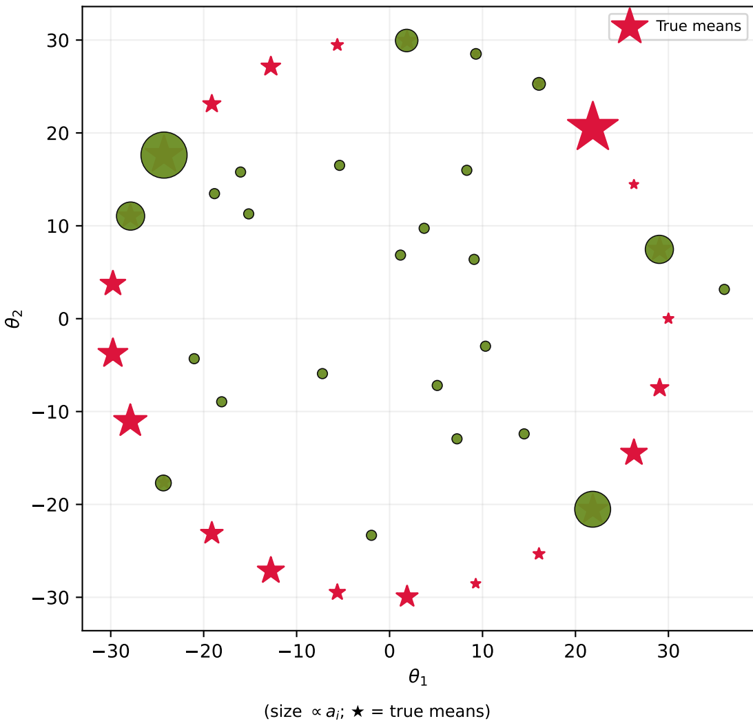
Stochastic CPGD (no BD) ( p=25 )
