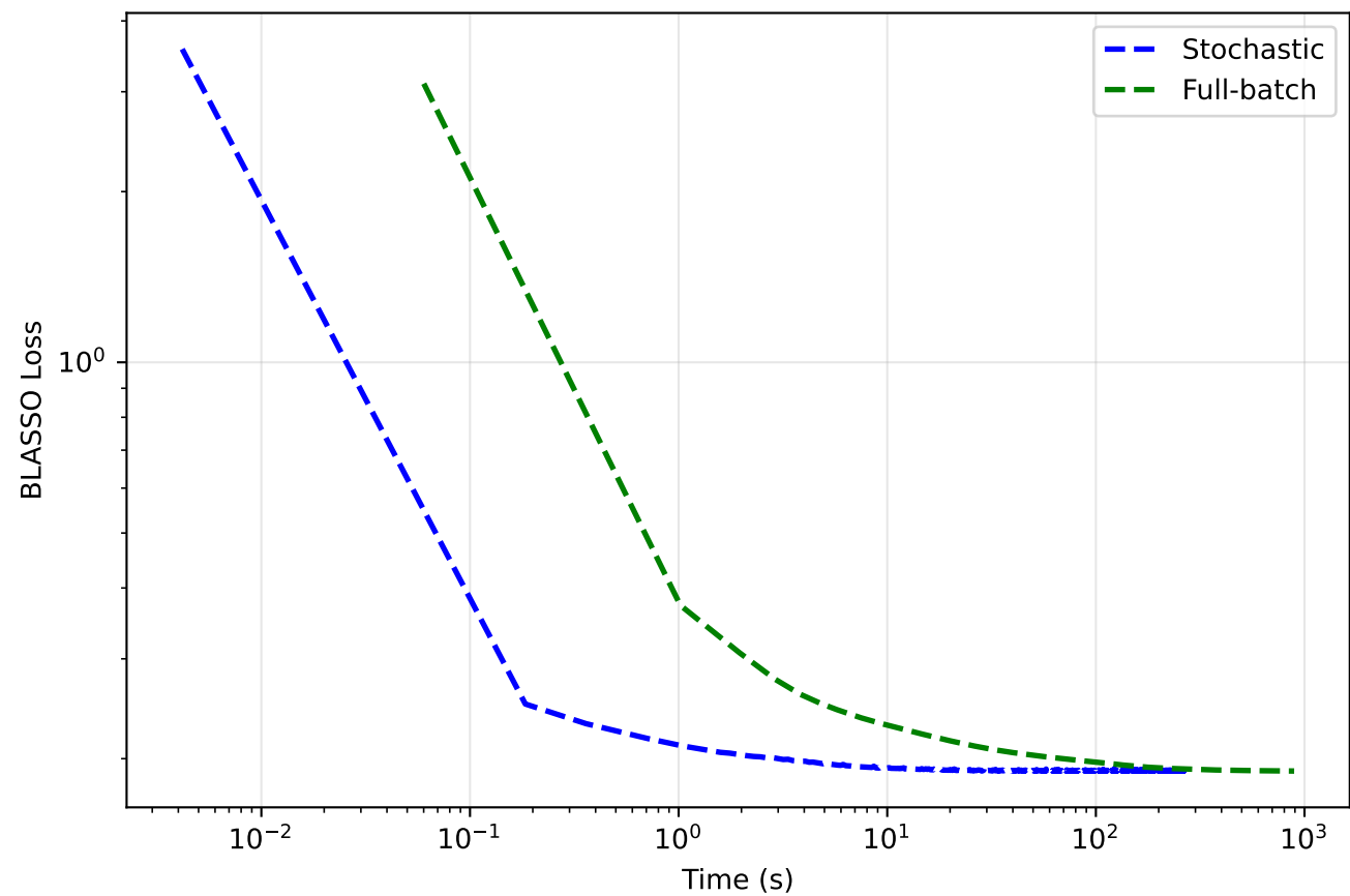
BLASSO Loss vs Wall-Clock Time
