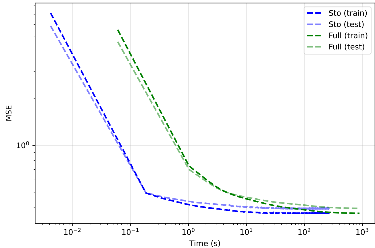
MSE vs Wall-Clock Time
