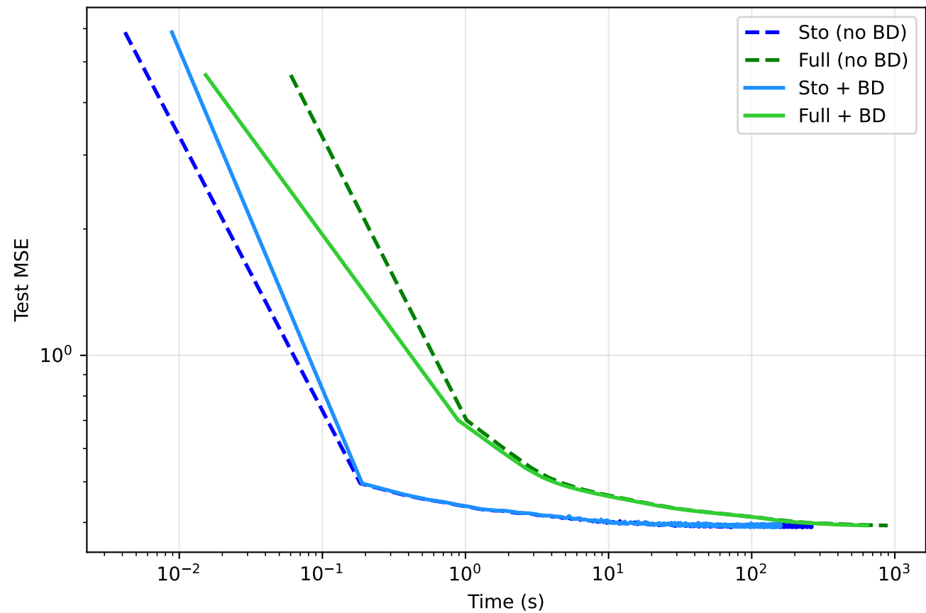
Test MSE vs Wall-Clock Time
