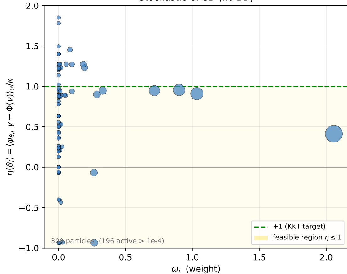
Stochastic CPGD (no BD)
