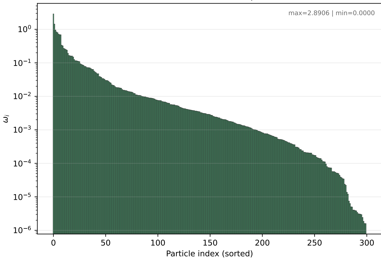
Full-Batch CPGD (no BD) (p=300)
