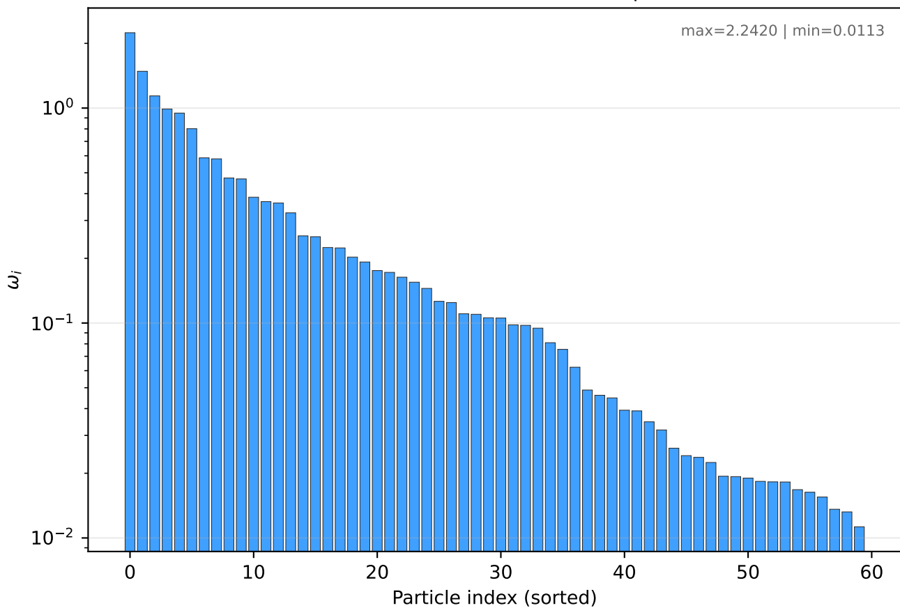
Stochastic CPGD + Birth-Death (p=60)
