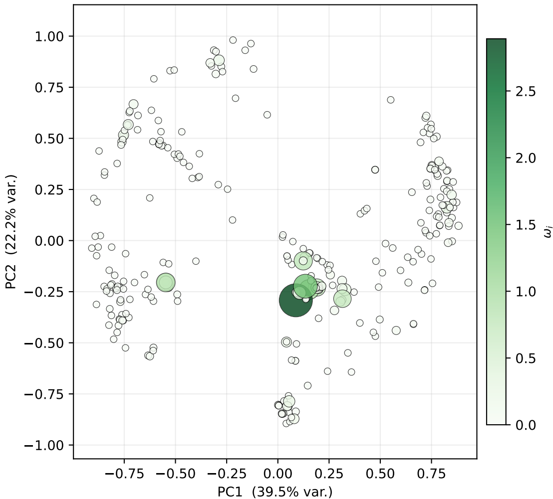
Full-Batch CPGD (no BD) ( p=300 )
