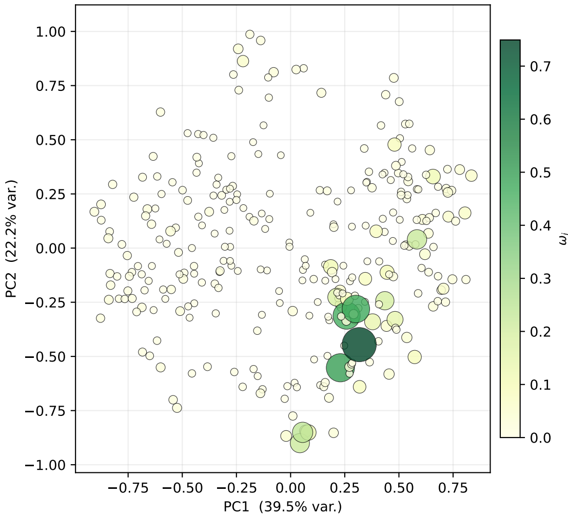
Full-Batch CPGD + Birth-Death ( p=300 )
