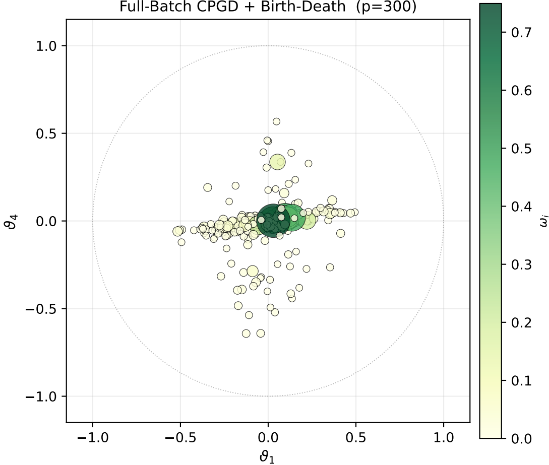
Full-Batch CPGD + Birth-Death ( p=300 )
