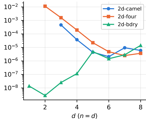
(c) f^* - \text{LBcert} (positive: valid)
