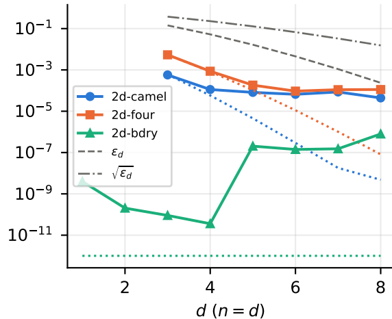
(b) distance to arg minf
