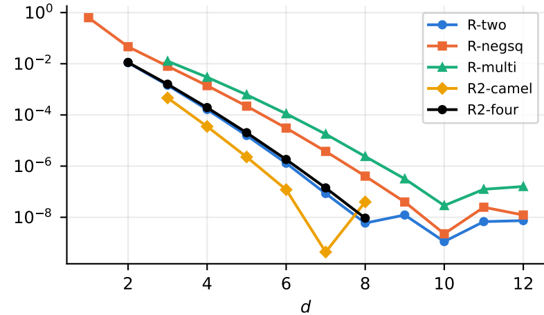
|\rho_d - f^*| on \mathbb{R}^p
