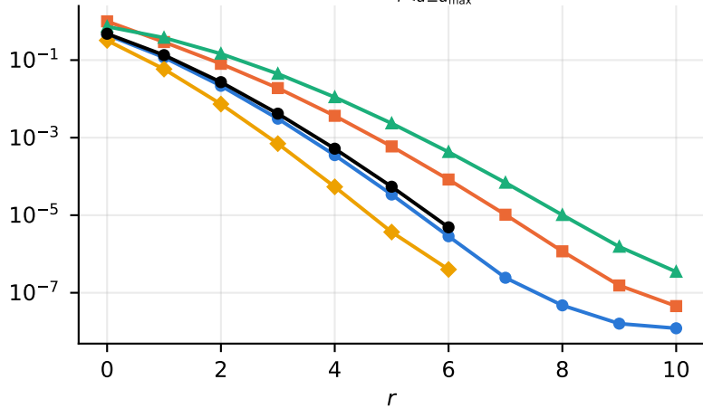
tightness (T): \sup_{r < d \leq d_{\max}} T(r; d)
