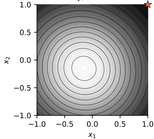
2d-bdry, f^* = 0.1353
