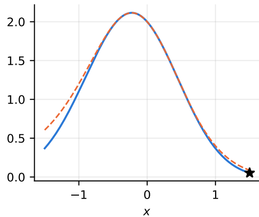
1d-bdry, f^* = 0.0527
