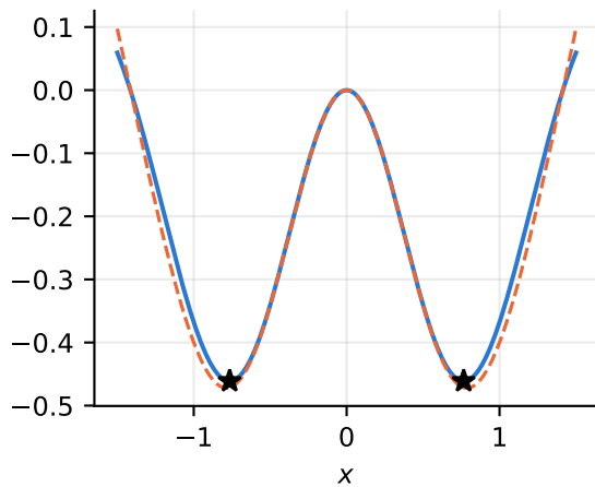
1d-two, f^* = -0.4612
