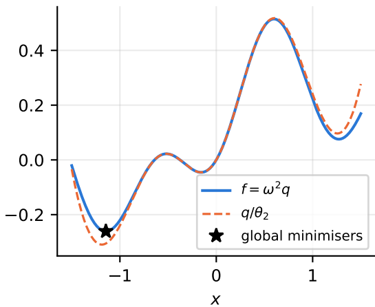
1d-multi, f^* = -0.2609
