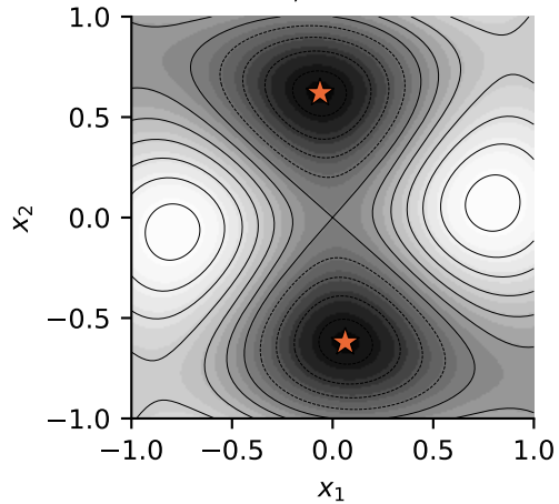
2d-camel, f^* = -0.6577
