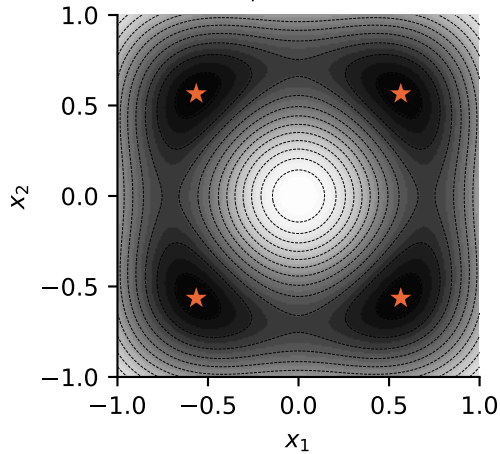
2d-four, f^* = -0.3712
