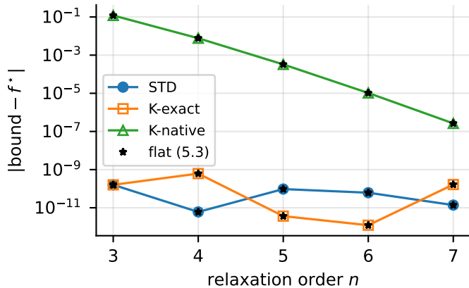
(a) six-hump camel, p = 2
