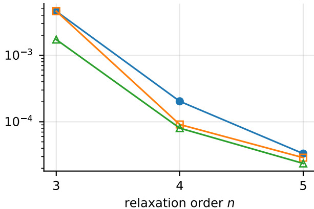
(b) Motzkin form on the ball, p = 3
