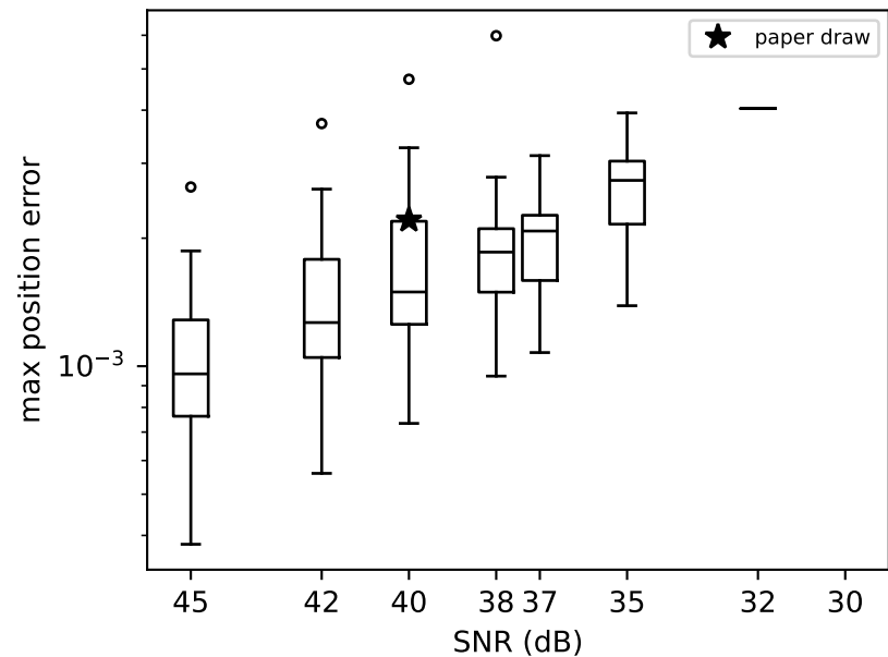
(c) accuracy of the successful draws
