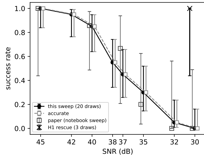
(a) signed recovery against noise
