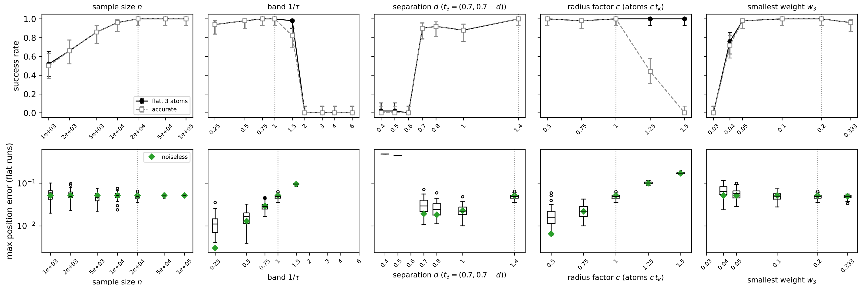
$6.5 mixture: 50 seeds per point (band 1, n = 2 \times 10^4 , d = 1.4 , w_3 = 0.2 unless varied)
