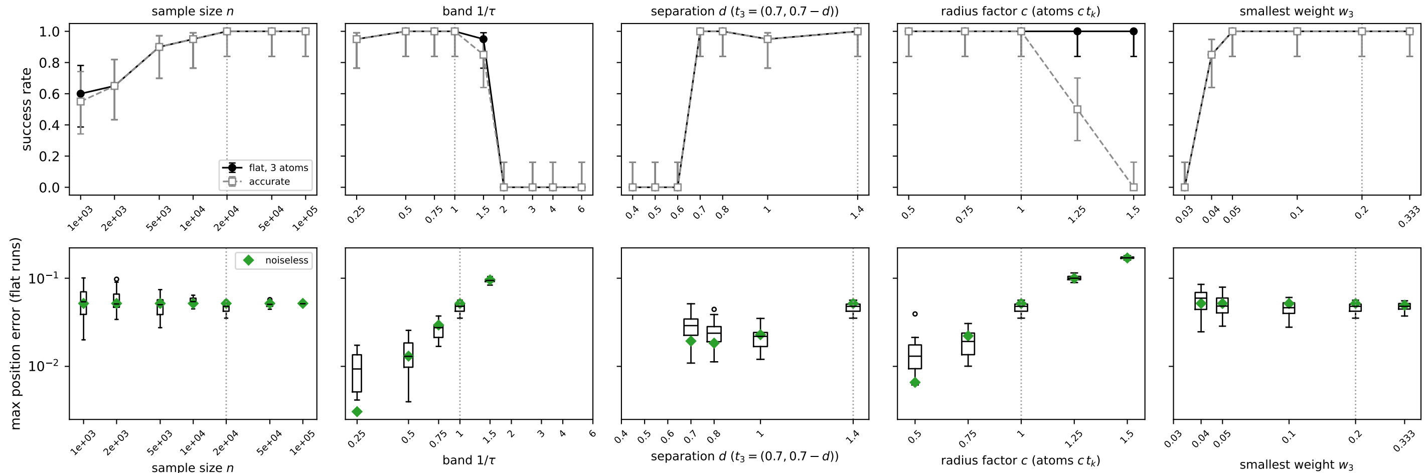
$6.5 mixture: 20 seeds per point (band 1, n = 2 \times 10^4 , d = 1.4 , w_3 = 0.2 unless varied)
