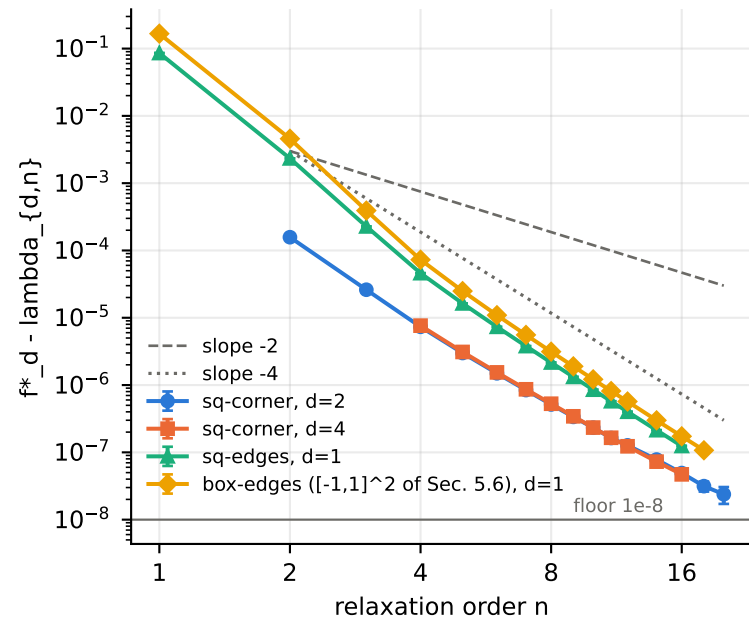
(a) Putinar module, zeros at a vertex (with the product g_1 g_2 : exact, < 1e-8 )
