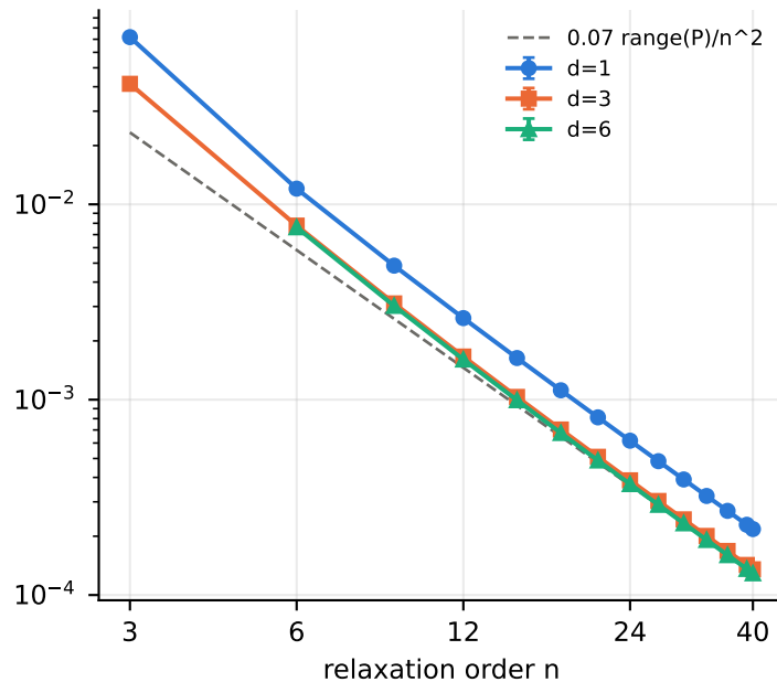
(b) positive control: [-1.5, 1.5] described by (2.25-x^2)^3 \geq 0 only (Stengle)
