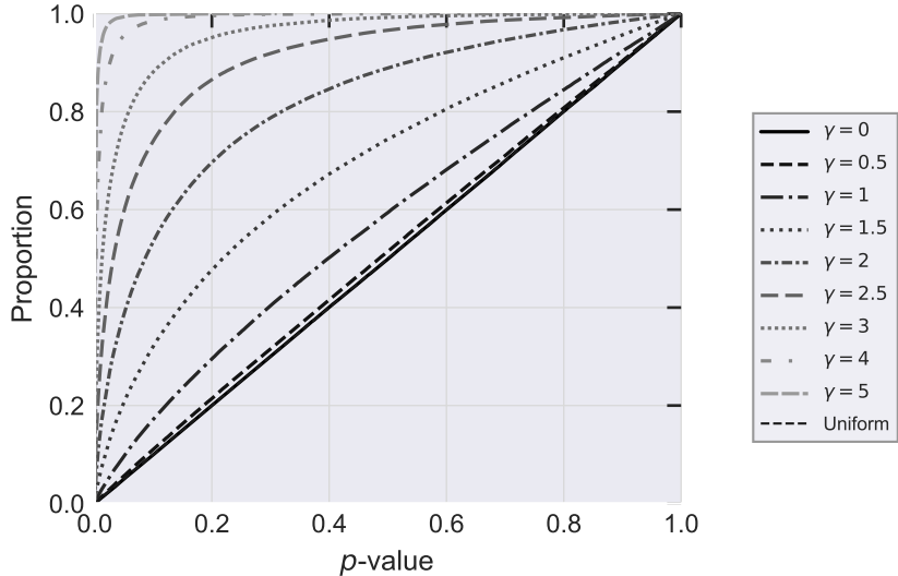
t -Spacing test ( \sigma unknown)
