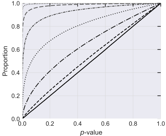
Spacing test ( \sigma known)
