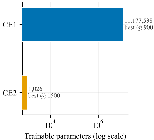
Fine-tuning efficiency
