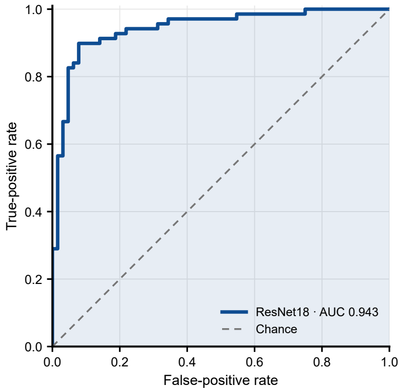
CHNCXR test-set ROC
