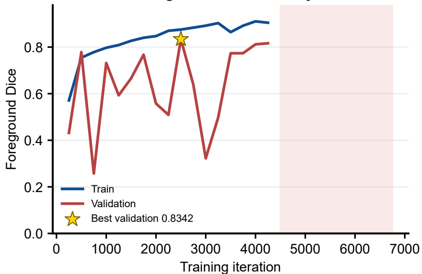
Segmentation accuracy
