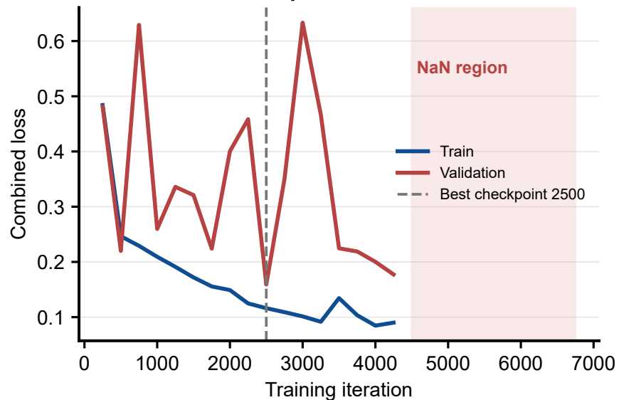
Optimization
