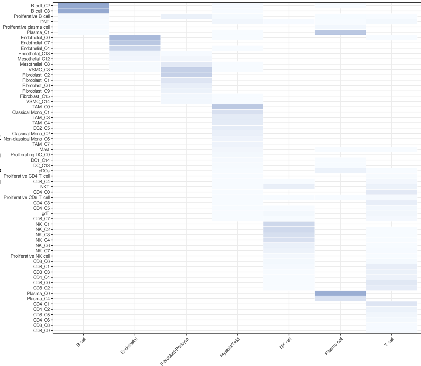
Original cells: blind annotation vs held-out original celltype
