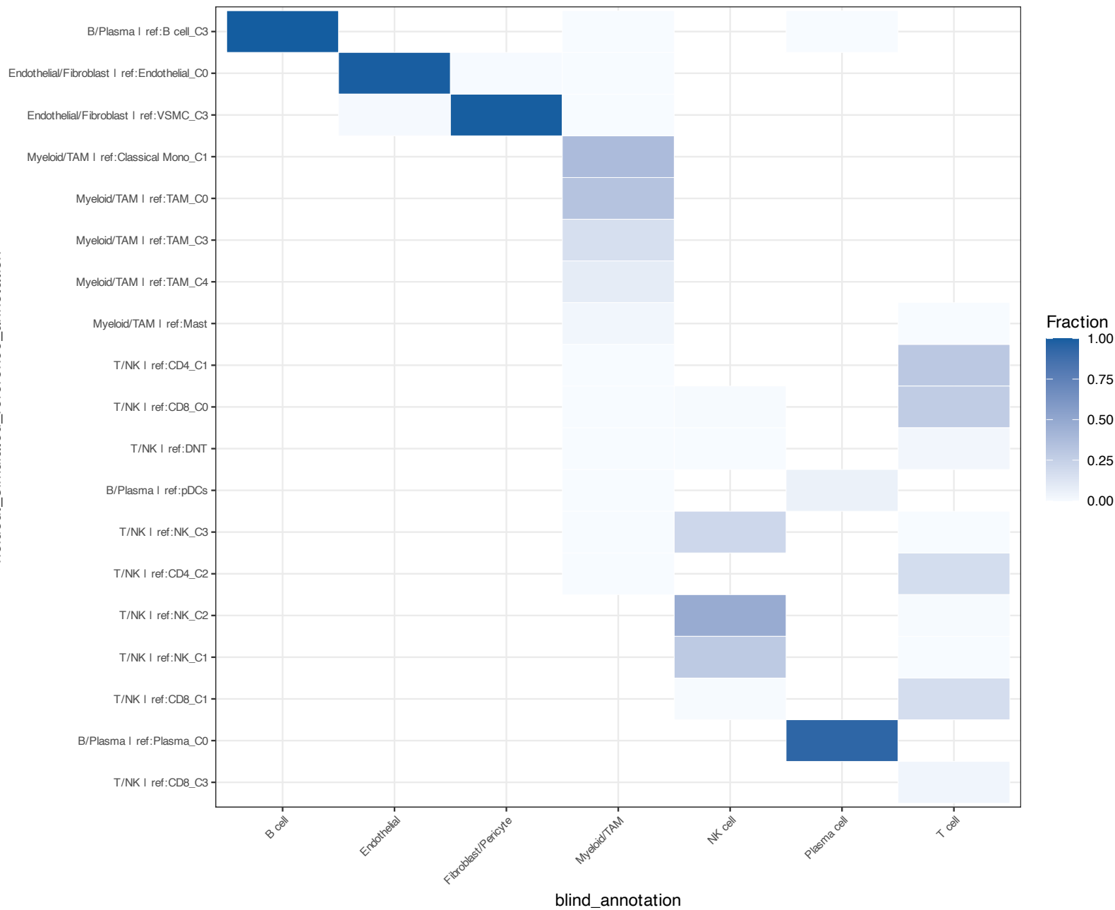
Simulated cells: blind annotation vs held-out reference label
