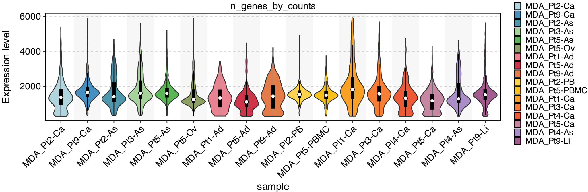
GSE234129 QC metrics by sample
