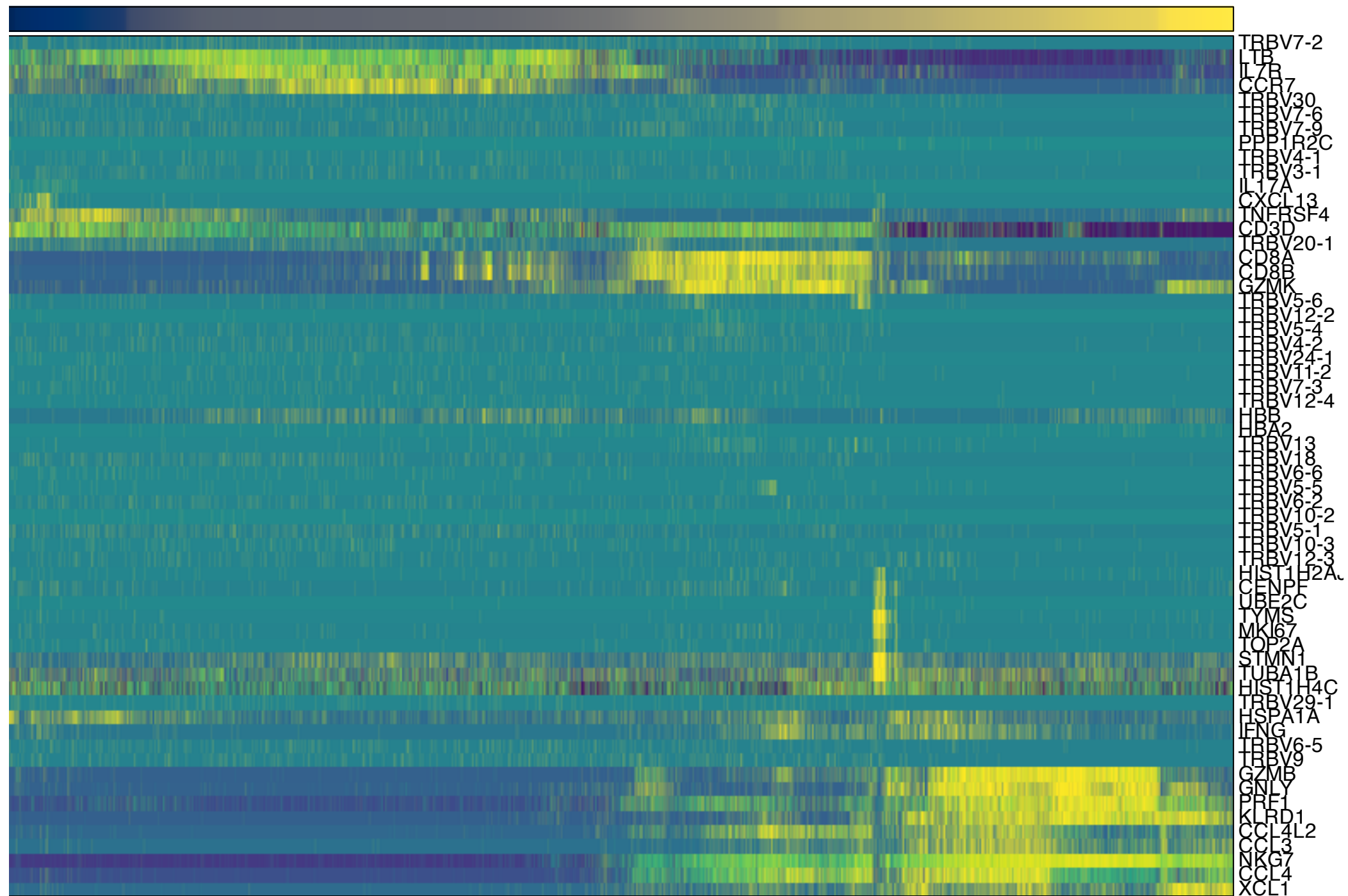
t_nk_Lineage1
