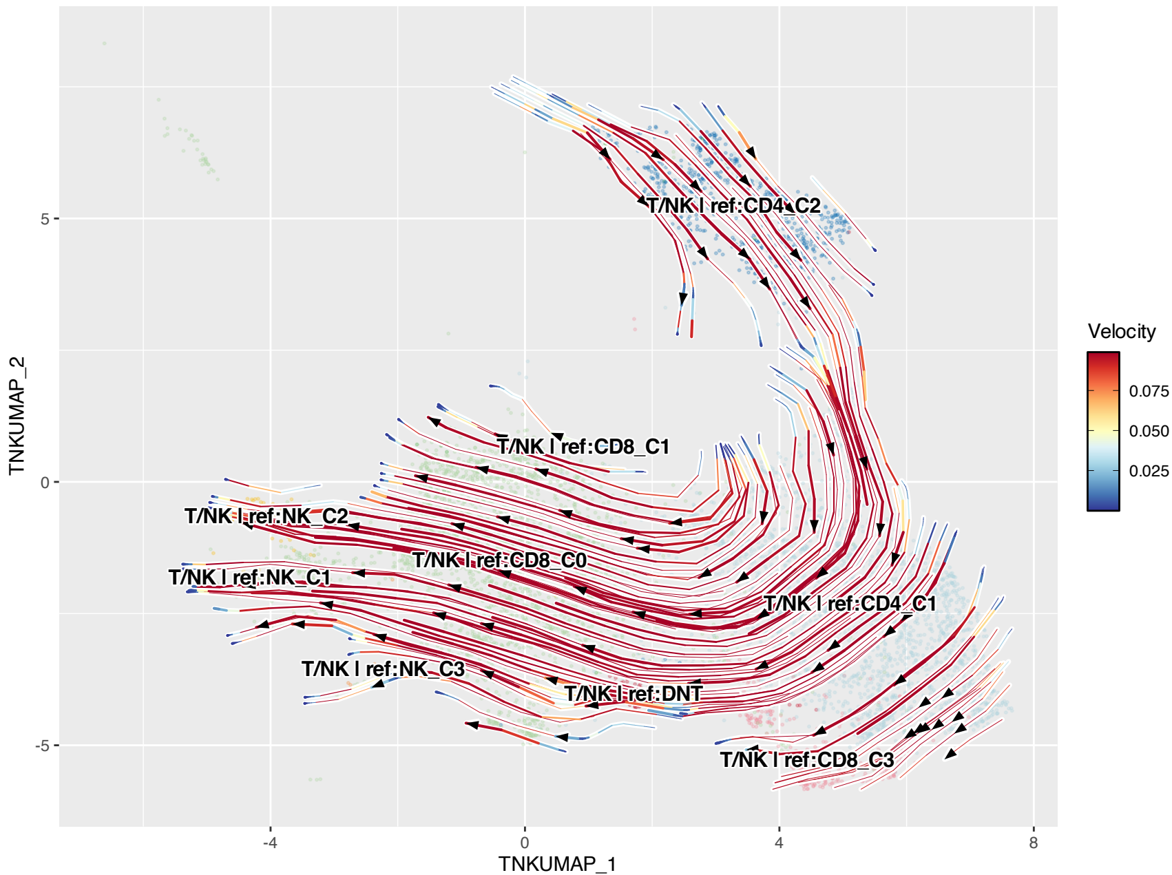
T/NK t_nk_Lineage3 projection
