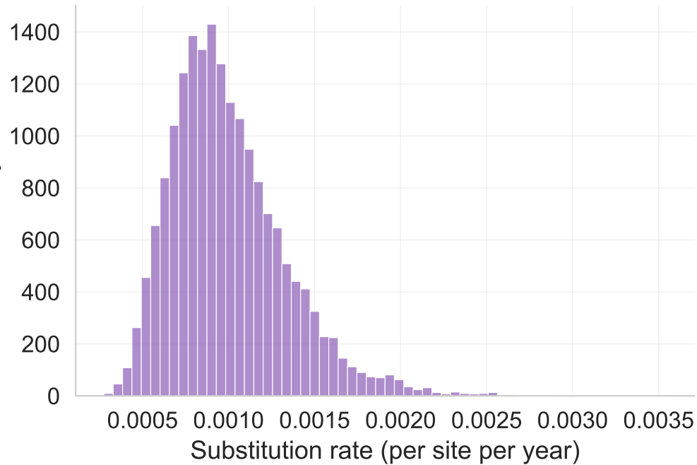
Clock rate distribution
