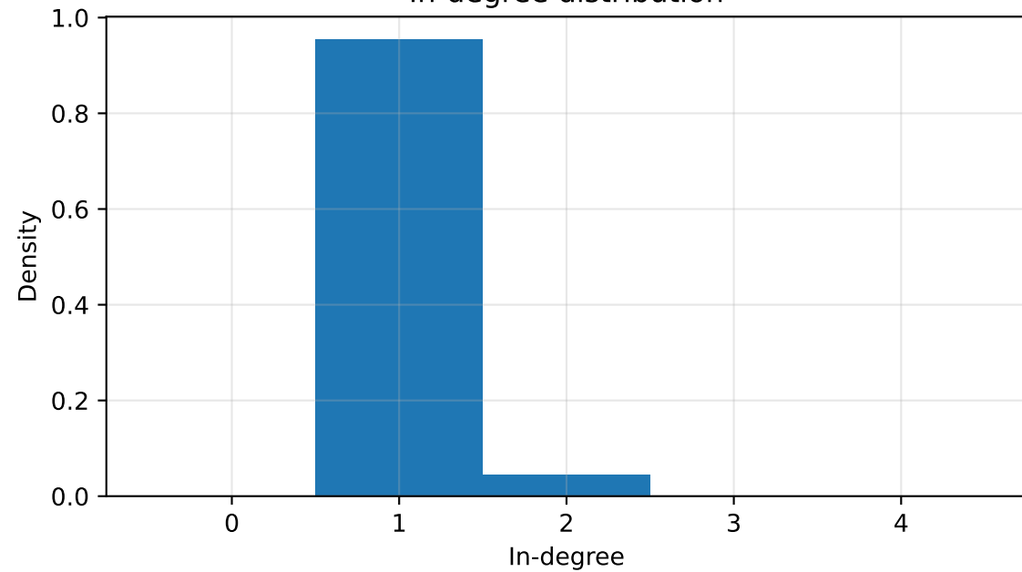
In-degree distribution
