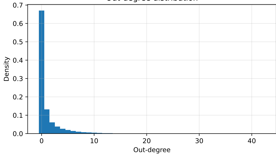
Out-degree distribution
