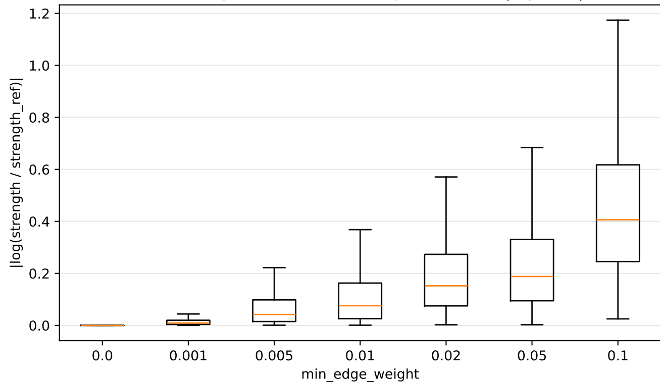
Node strength distortion under sparsification ( |\log \text{ratio}| )
