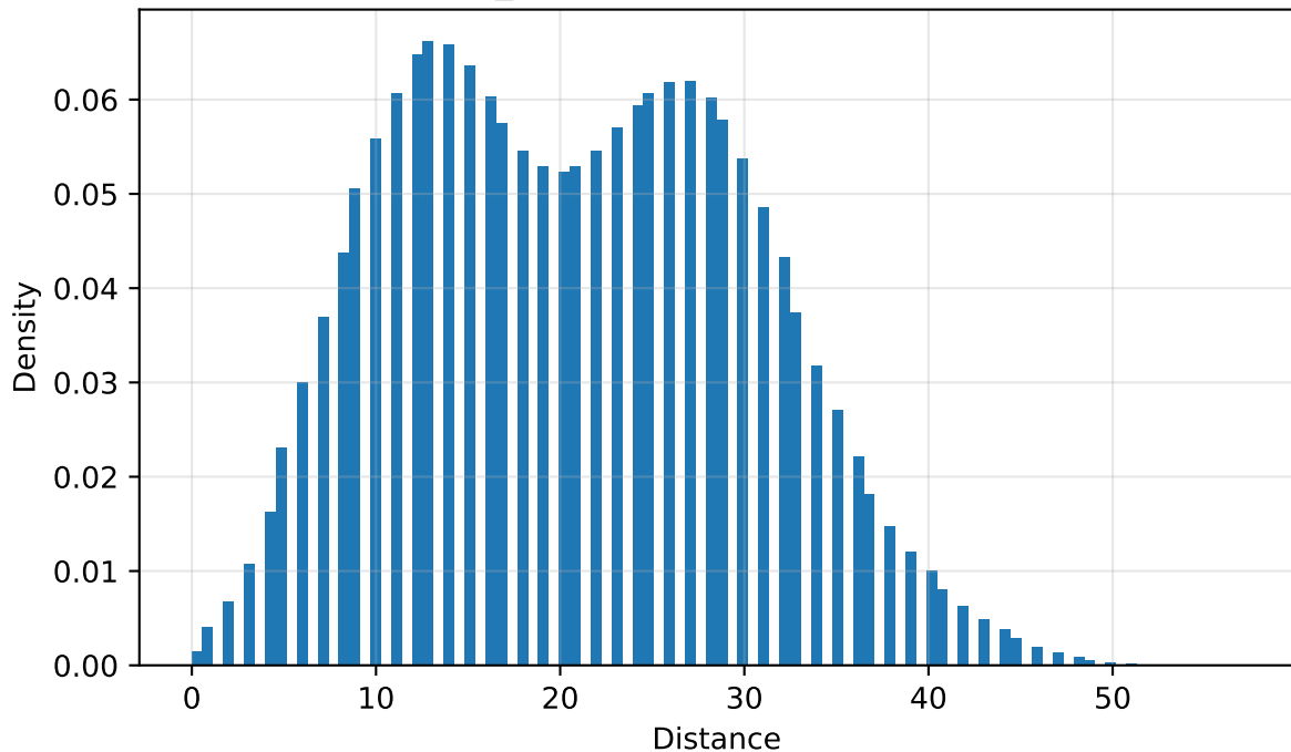
surveillance_moderate: Poisson Genetic distance
