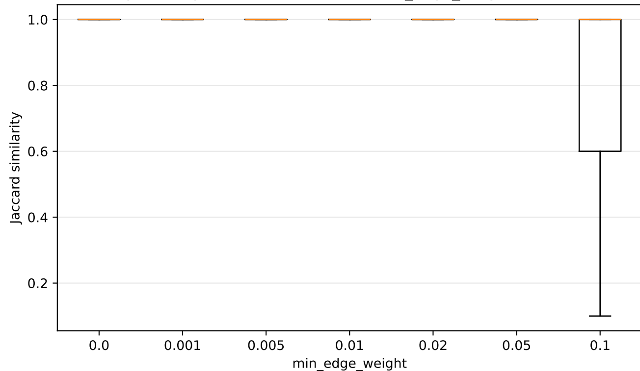
Top-20 neighbourhood Jaccard vs min_edge_weight (ref=0.0)
