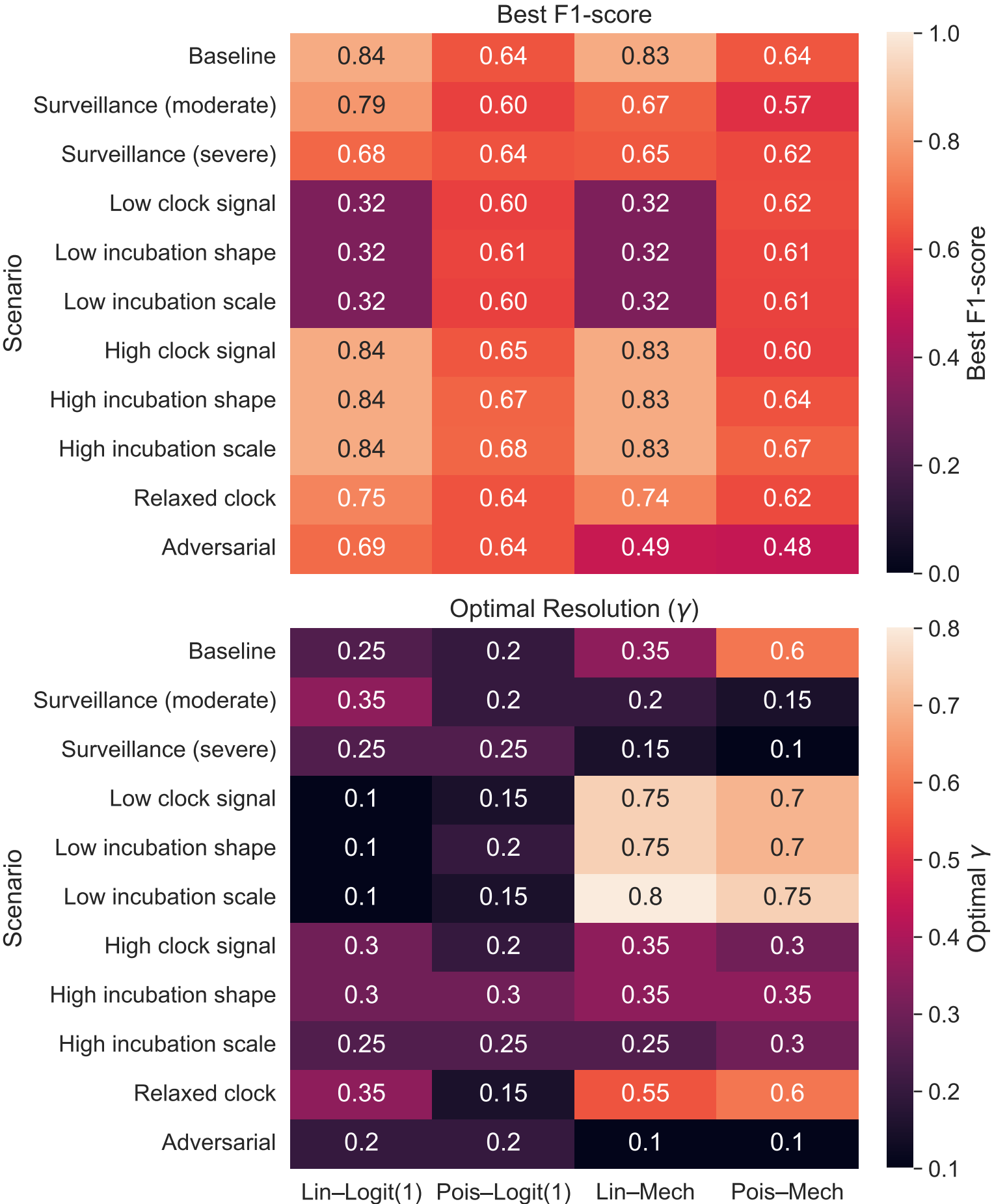
Best F1 score and \gamma across scenarios and models
