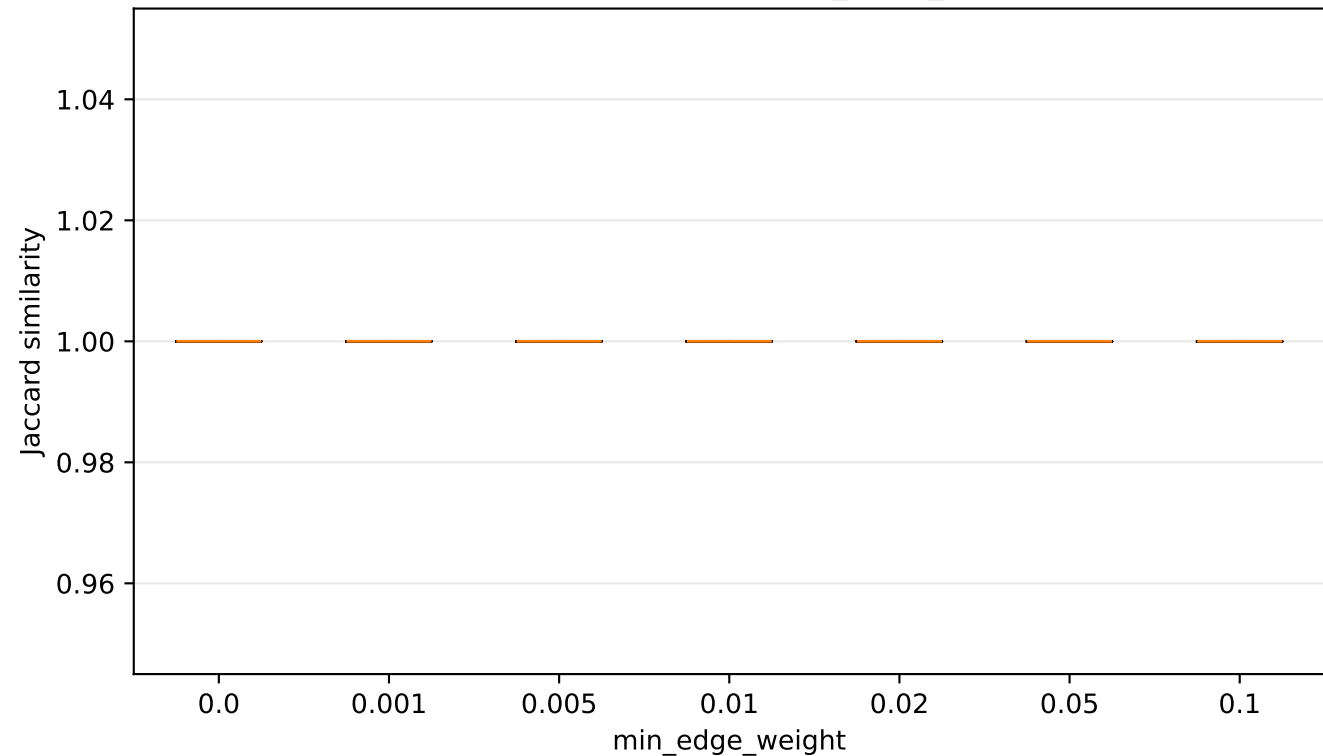
Top-5 neighbourhood Jaccard vs min_edge_weight (ref=0.0)
