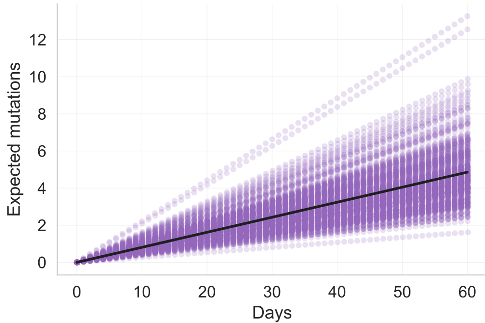
Expected mutations over time
