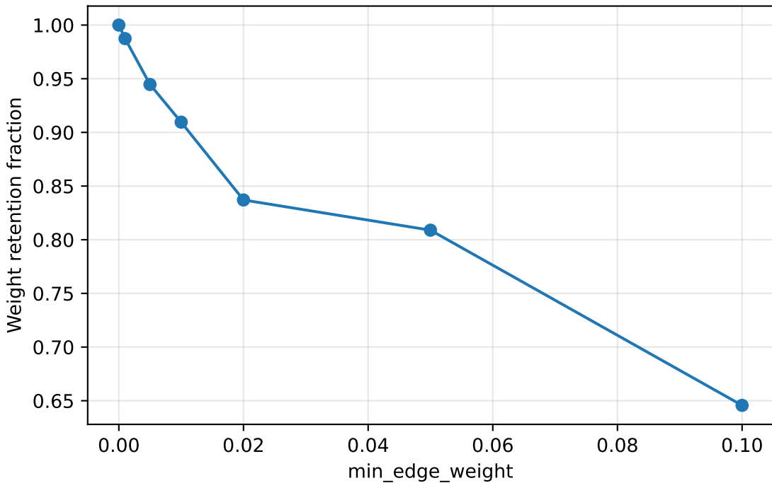
Total edge-weight retained under sparsification
