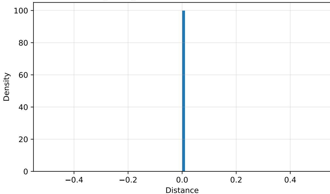
low_clock_signal: Linear Genetic distance
