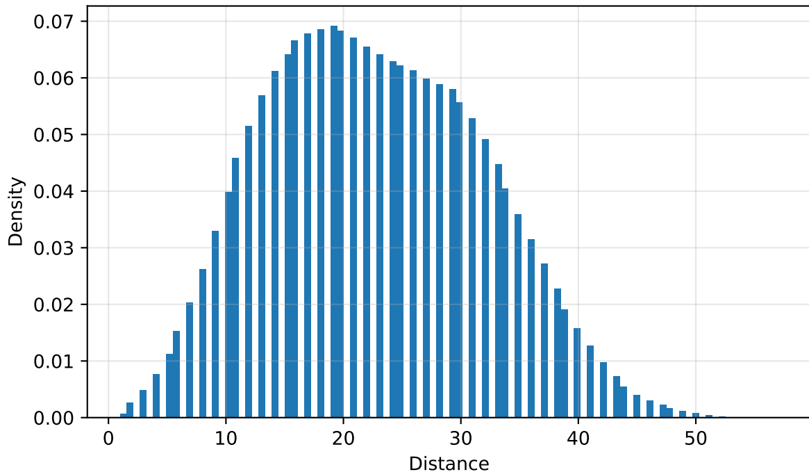
baseline: Linear Genetic distance
