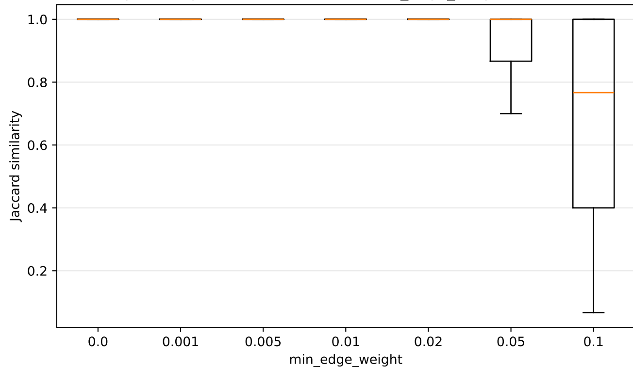
Top-30 neighbourhood Jaccard vs min_edge_weight (ref=0.0)
