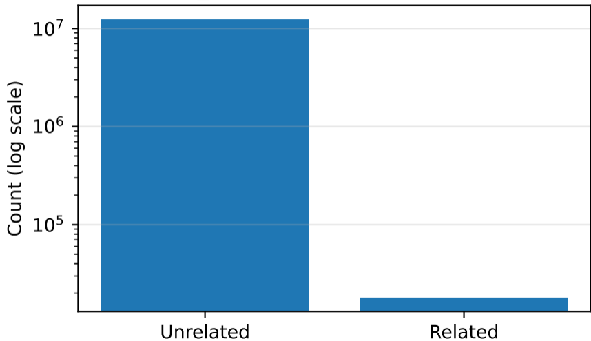
relaxed_clock: Class balance (Sampled)
