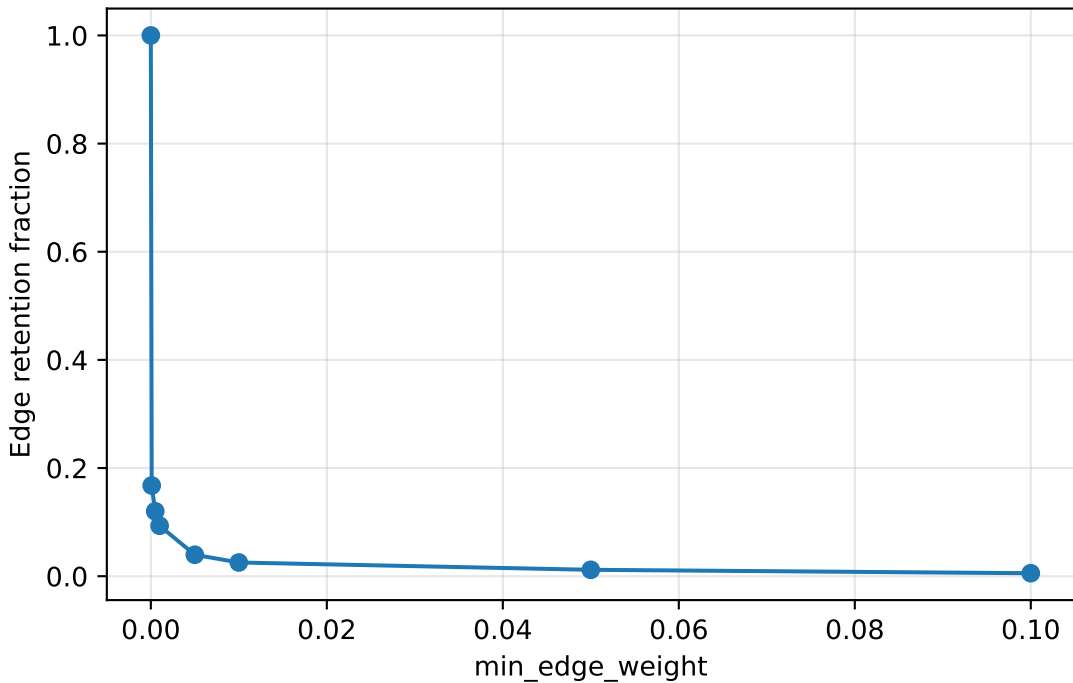
Edge count retained under sparsification
