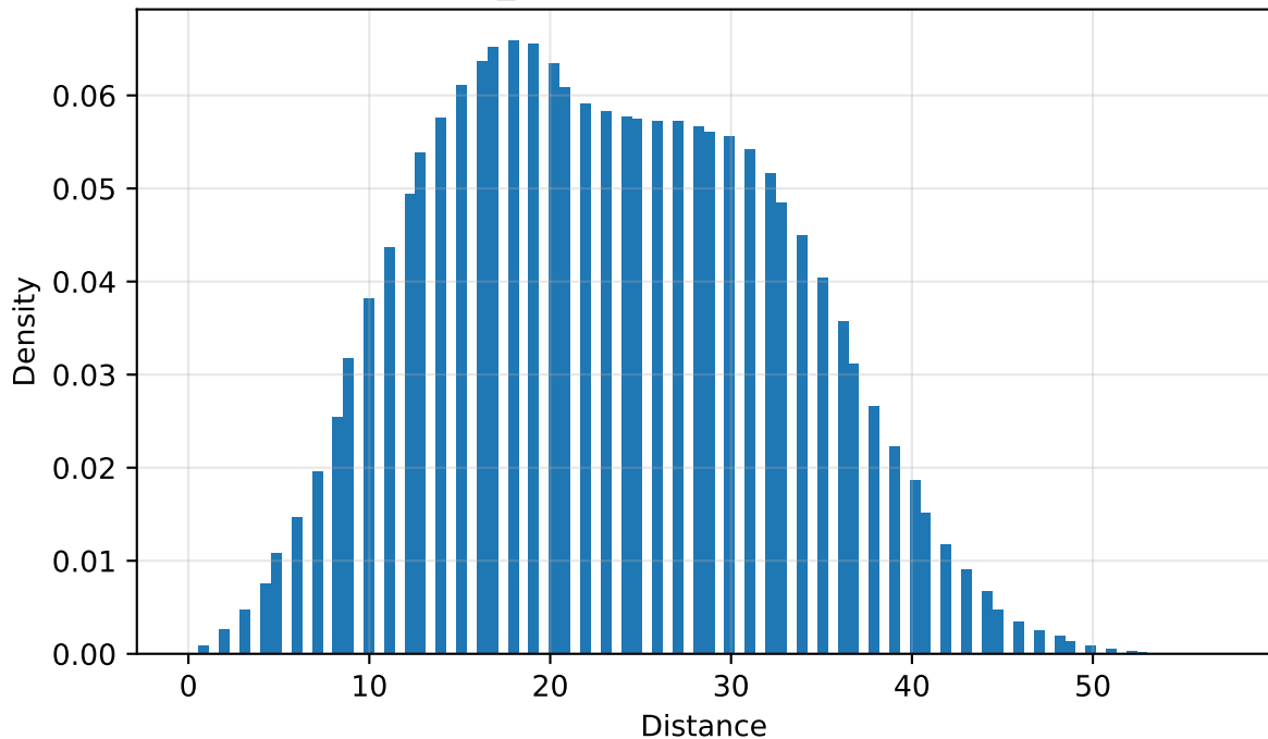
surveillance_moderate: Linear Genetic distance
