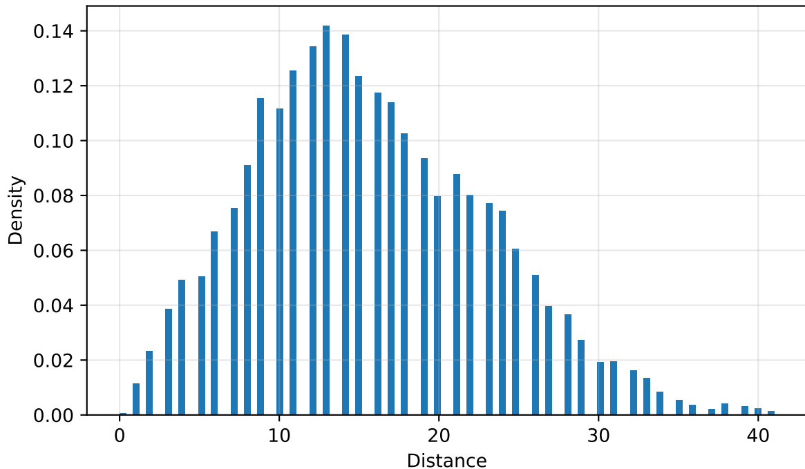
adversarial: Deterministic genetic distance
