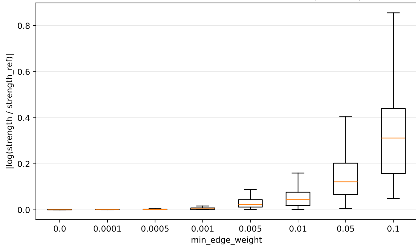
Node strength distortion under sparsification ( |\log \text{ratio}| )
