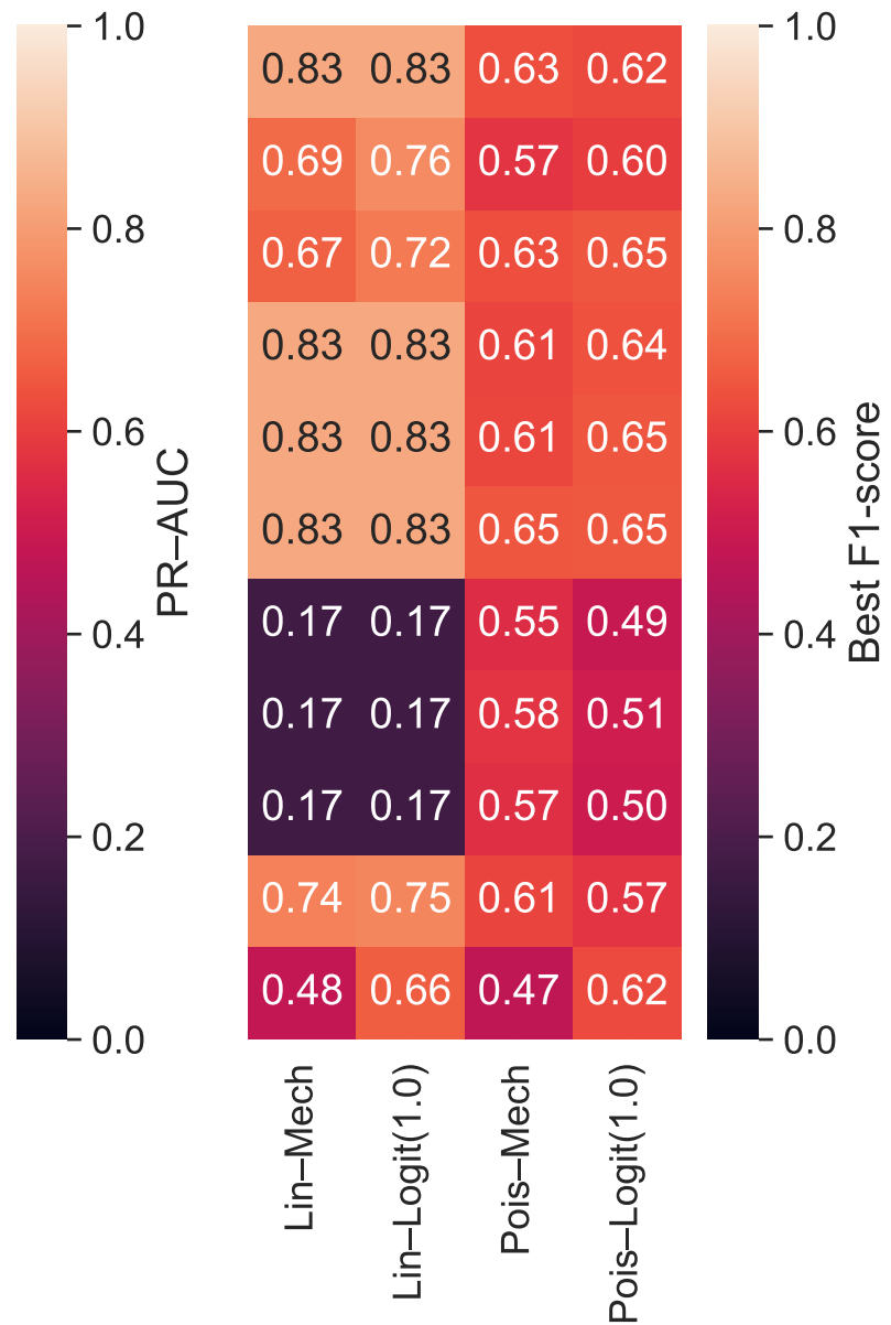
(b) Cluster recovery
