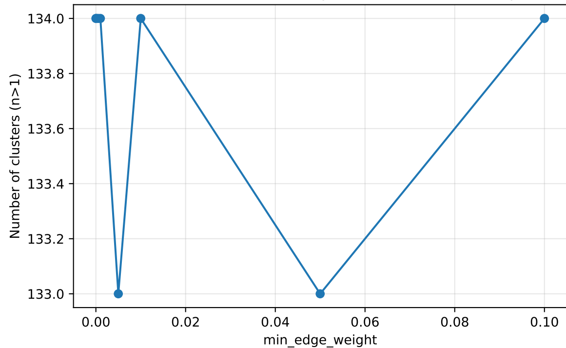
Number of Leiden clusters vs sparsification threshold ( \gamma=0.5 )
