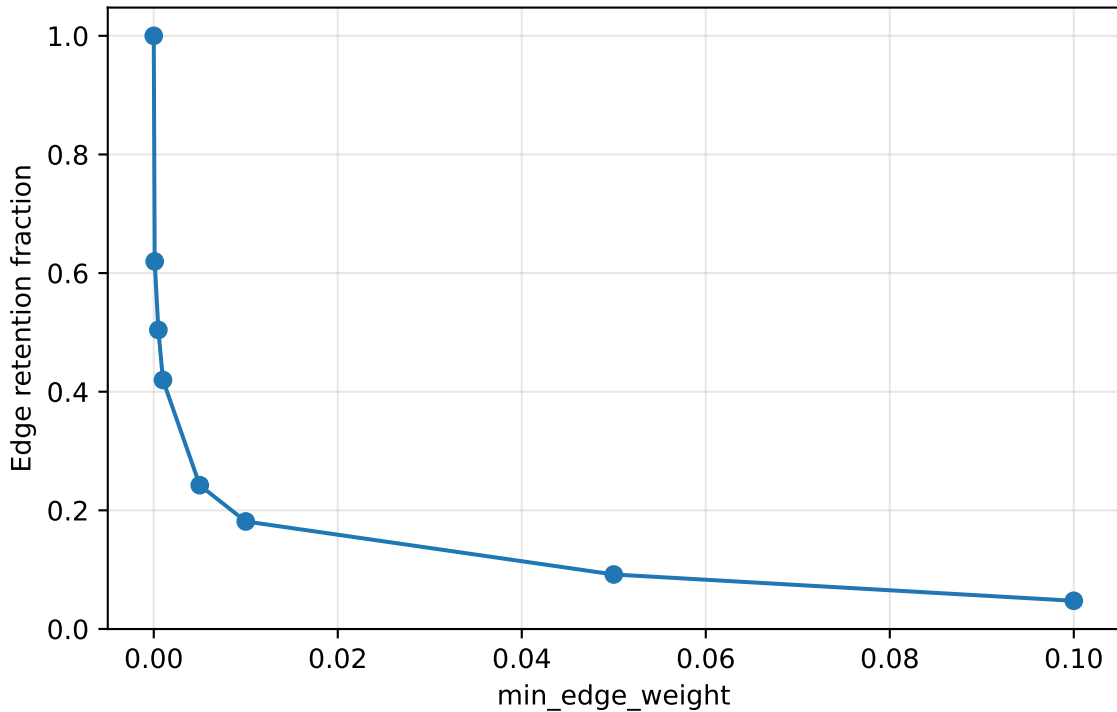
Edge count retained under sparsification
