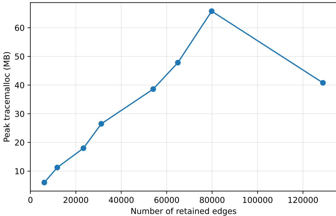
Peak Python-allocated memory vs retained edges
