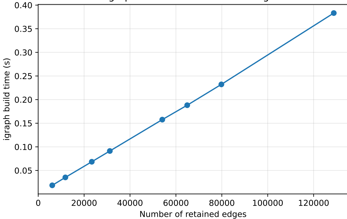
igraph build time vs retained edges
