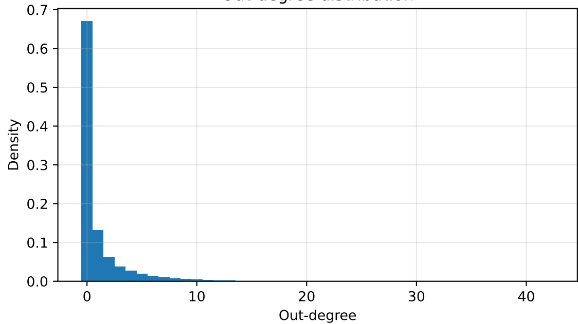
Out-degree distribution
