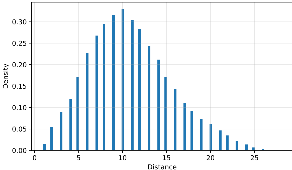
high_scale_inc: Deterministic genetic distance
