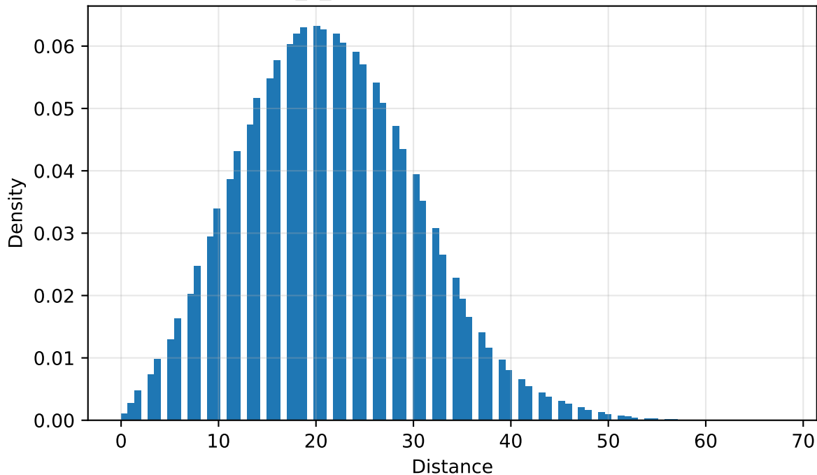
high_k_inc: Poisson Genetic distance
