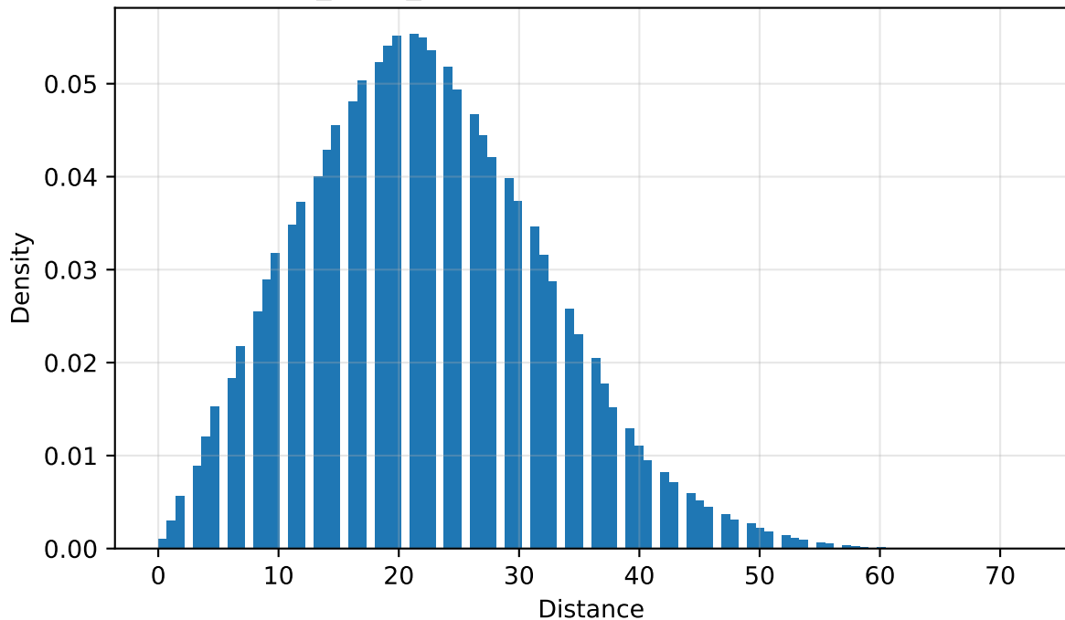
high_clock_signal: Stochastic genetic distance
