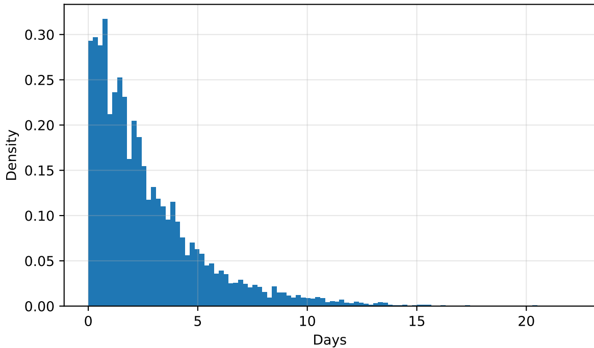
Time from onset of infectiousness to transmission (TOIT)
