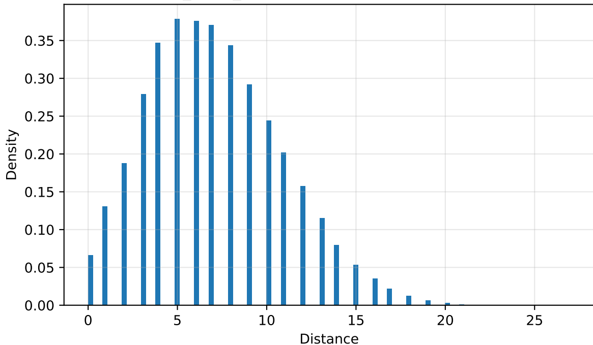
low_clock_signal: Poisson Genetic distance
