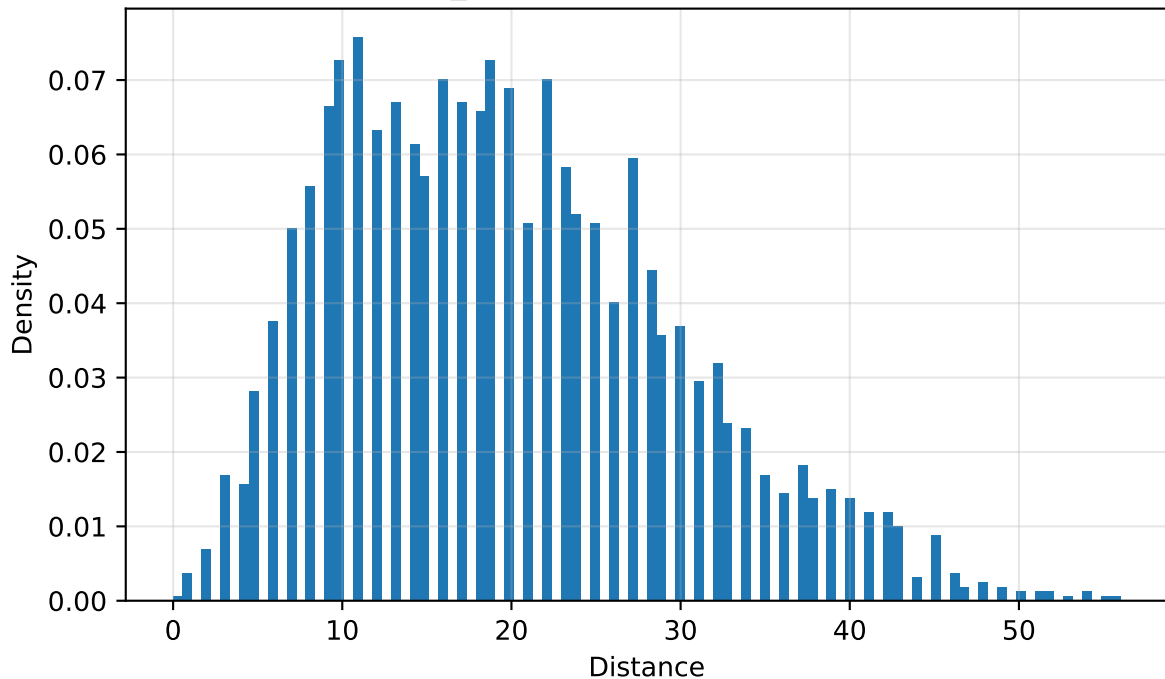
surveillance_severe: Stochastic genetic distance
