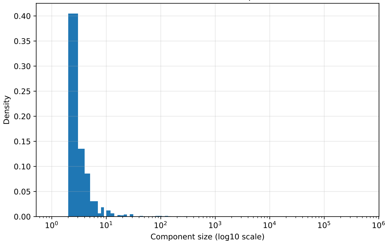
Distribution of connected component sizes
