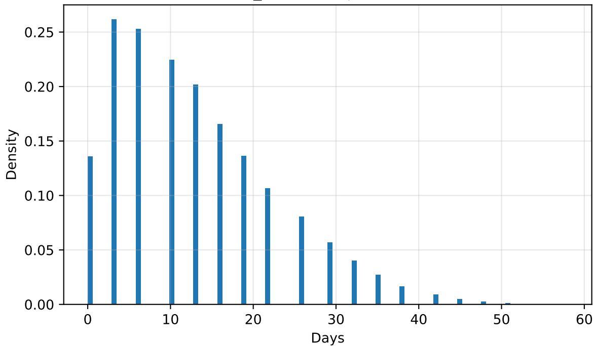
relaxed_clock: Temporal distance
