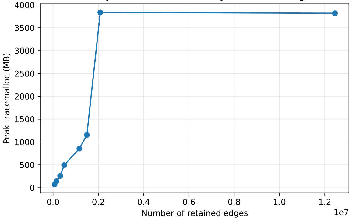
Peak Python-allocated memory vs retained edges
