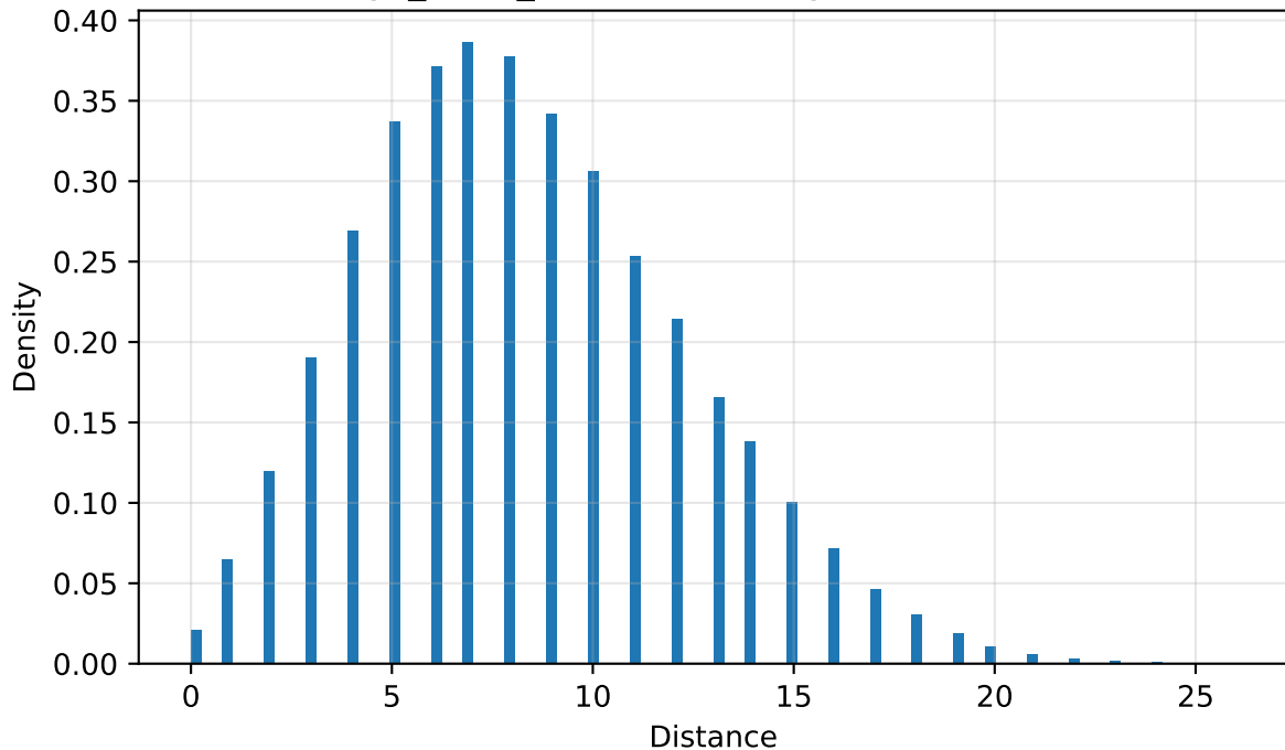
high_scale_inc: Stochastic genetic distance
