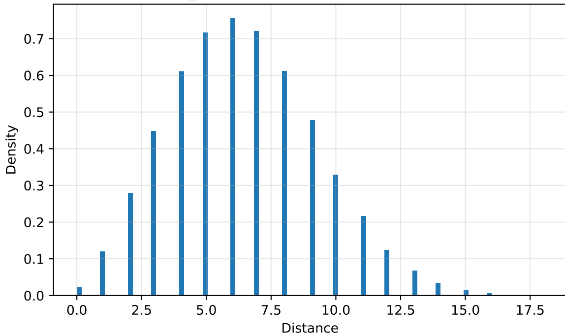
relaxed_clock: Deterministic genetic distance
