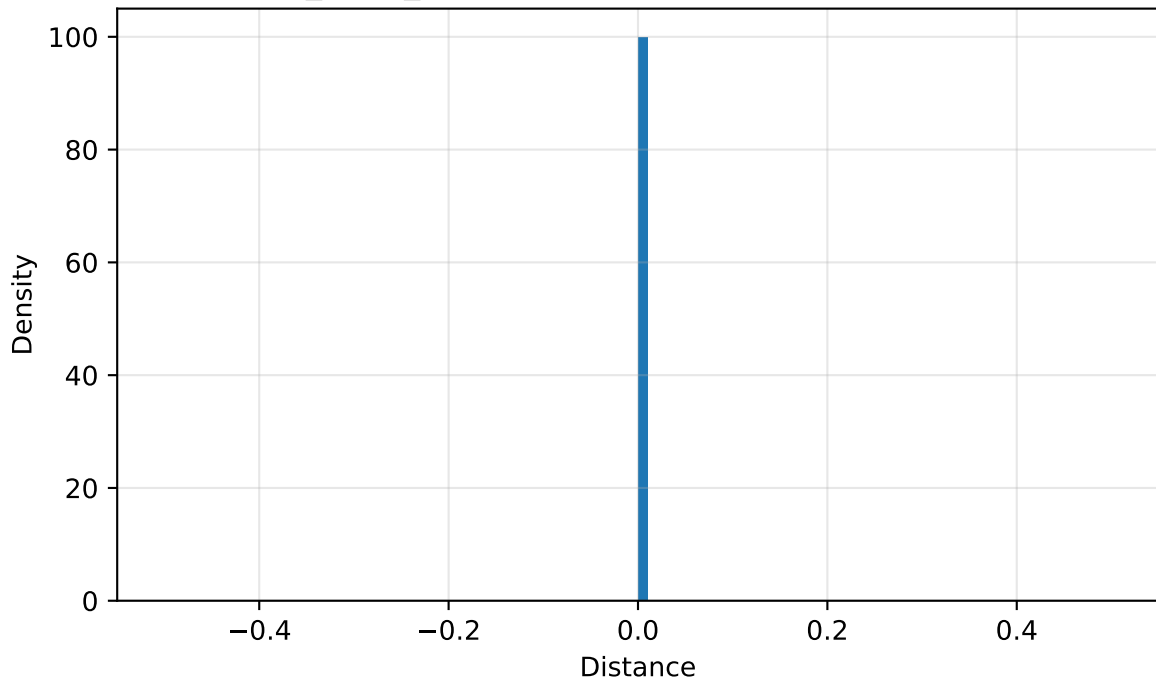
low_clock_signal: Deterministic genetic distance
