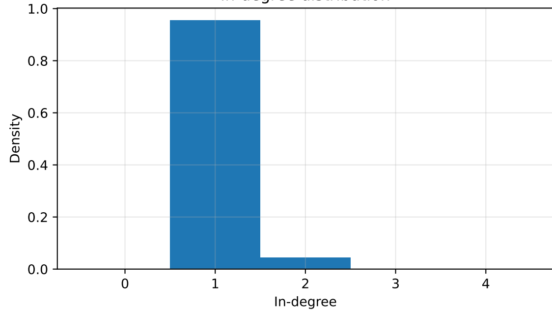
In-degree distribution
