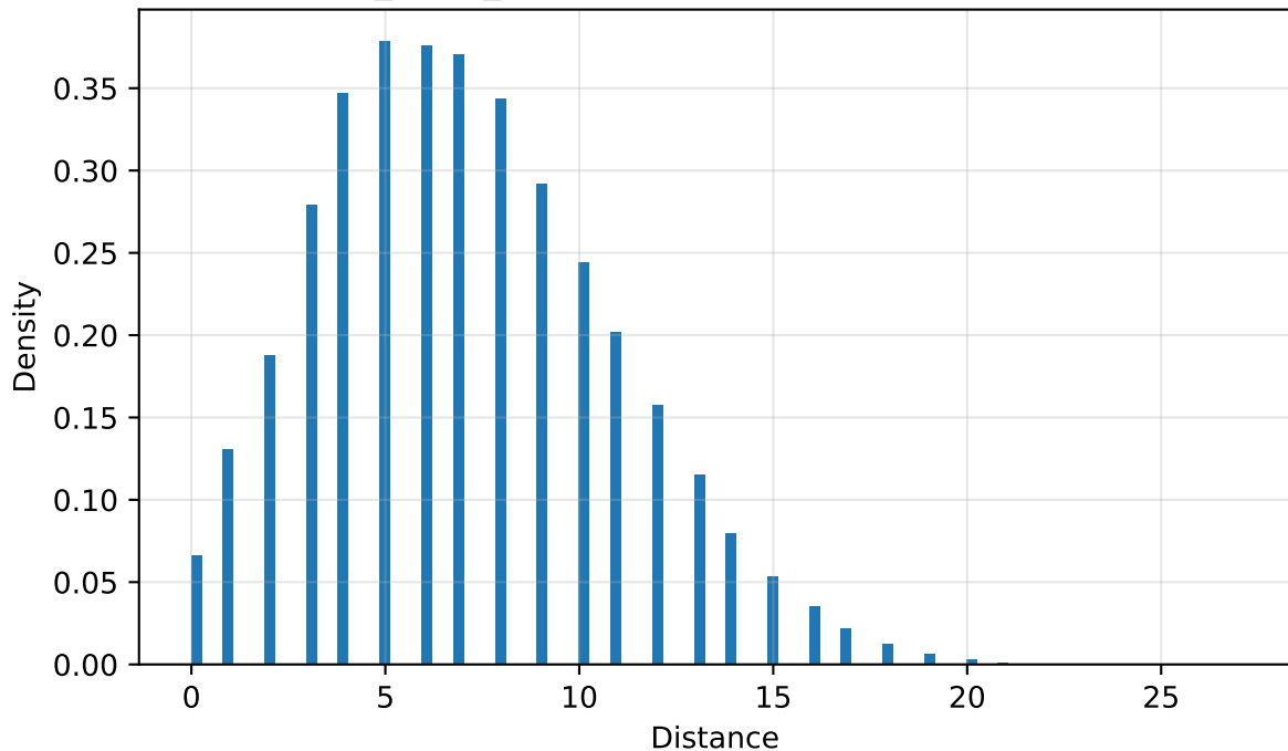
low_clock_signal: Stochastic genetic distance
