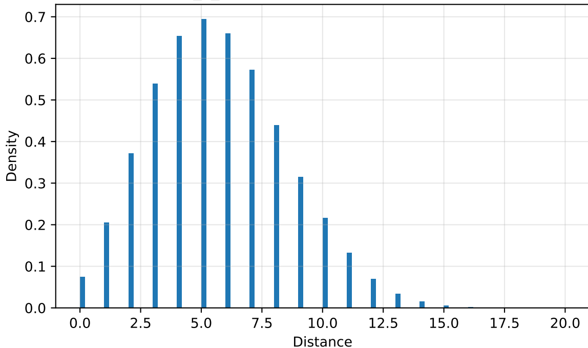
low_k_inc: Stochastic genetic distance
