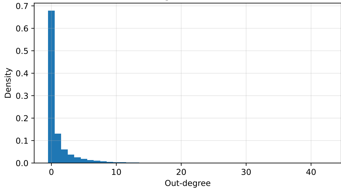
Out-degree distribution
