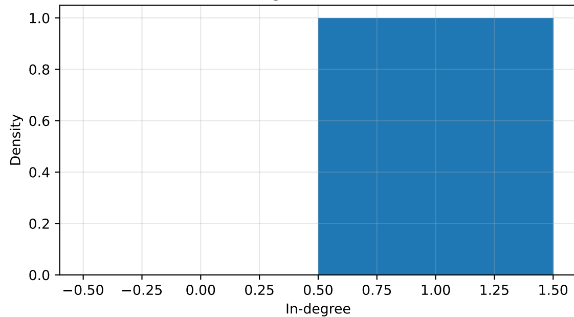
In-degree distribution
