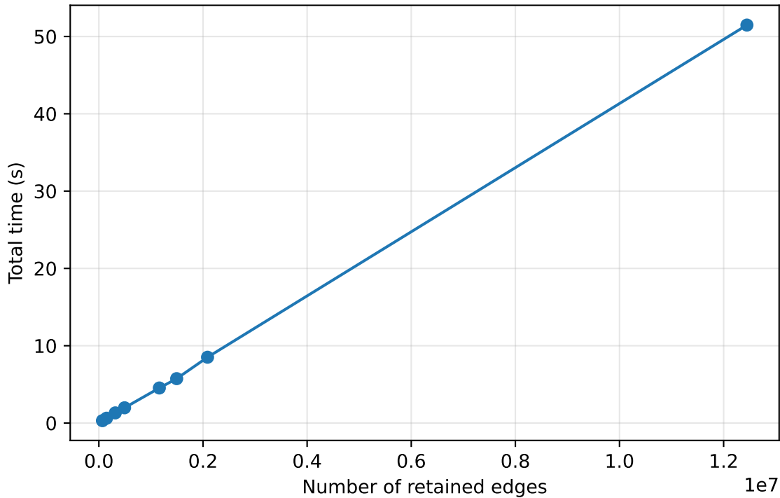
Wall-clock time vs retained edges (diagnostics)
