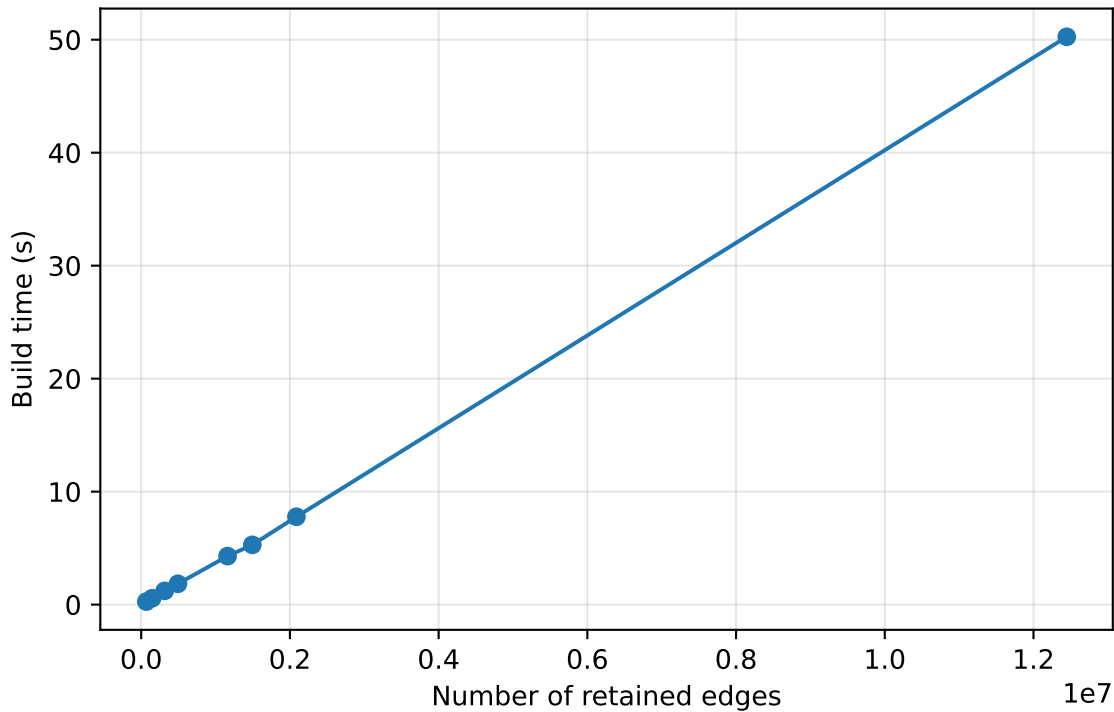
NetworkX graph build time vs retained edges
