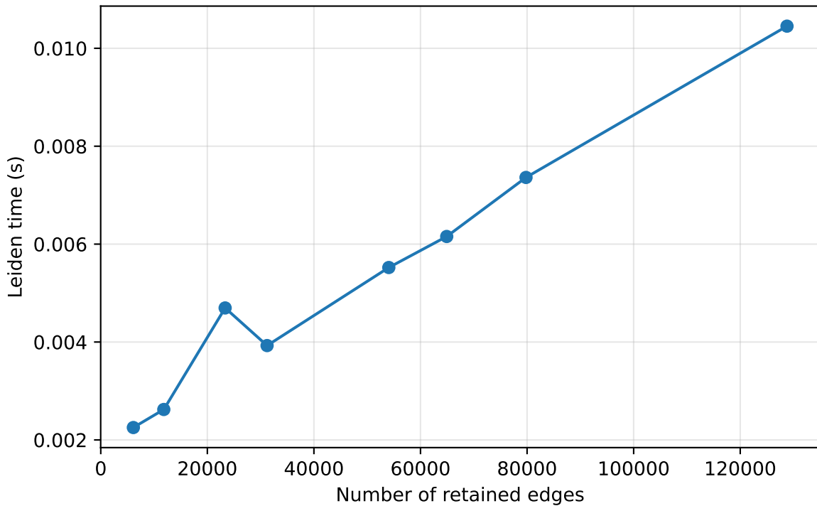
Leiden runtime vs retained edges ( \gamma=0.5 )
