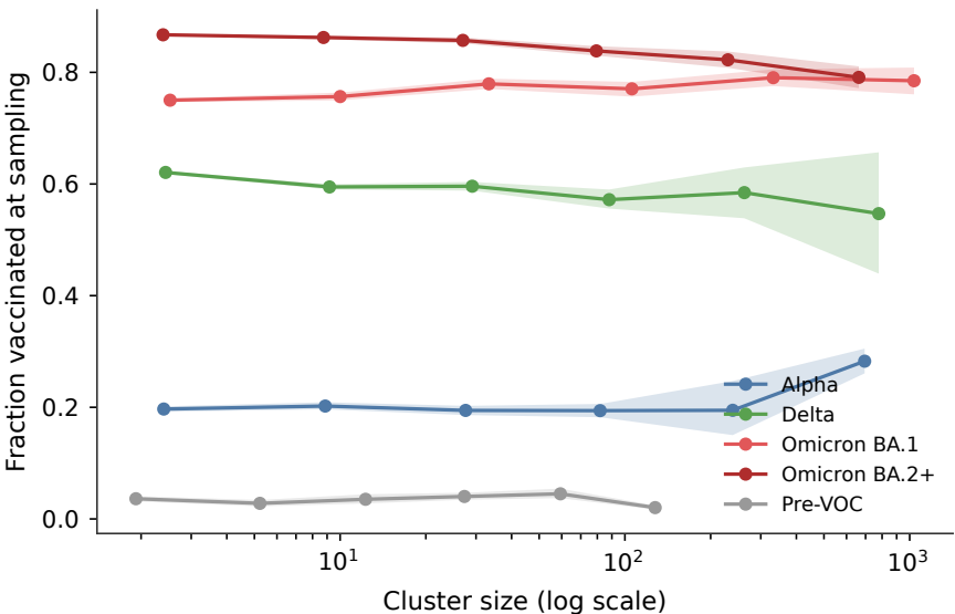
Vaccination prevalence vs. cluster size, by VOC epoch
