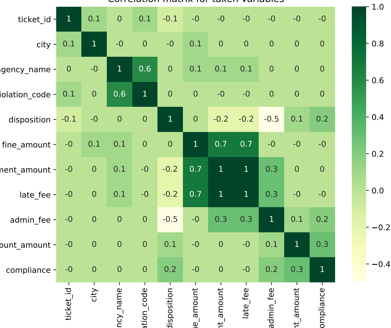
Correlation matrix for taken variables
